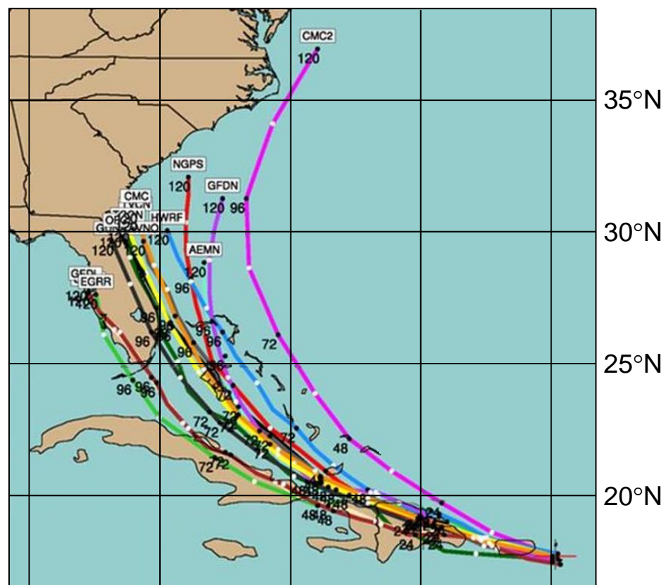
Hurricane Irene track forecasts, 08/22/11
