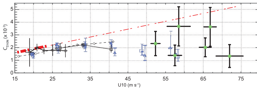
FIG. 19. Wind speed dependence of C_D from this study (green circles) compared with previous studies. Black symbols indicate data adapted from French et al. (2007) and blue symbols indicate data adapted from Vickery et al. (2009). Red line indicates measured (thick) and extrapolated (thin) Large and Pond (1981) drag coefficient.
