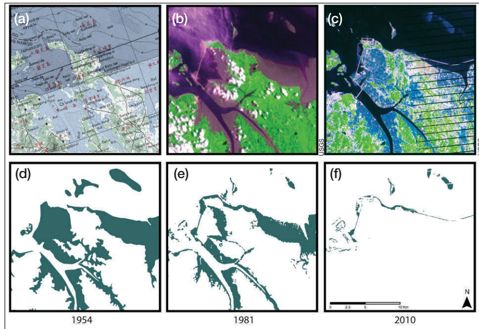
Figure 2. An example of tidal flat mapping results, showing the raw data (a–c) and mapped tidal flats (d–f). The results reveal widespread loss of tidal flats from 1954 (left) to 2010 (right). Satellite images (b) and (c) show that tidal flats present in 1981 (e) were reclaimed for agricultural and industrial land by 2010 (f).
