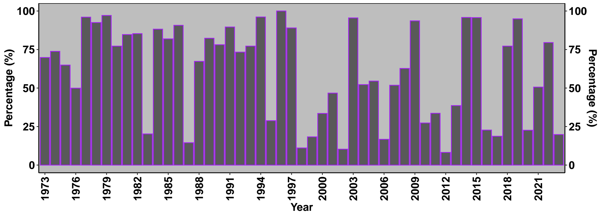
Lake Superior Annual Maximum Ice Cover
