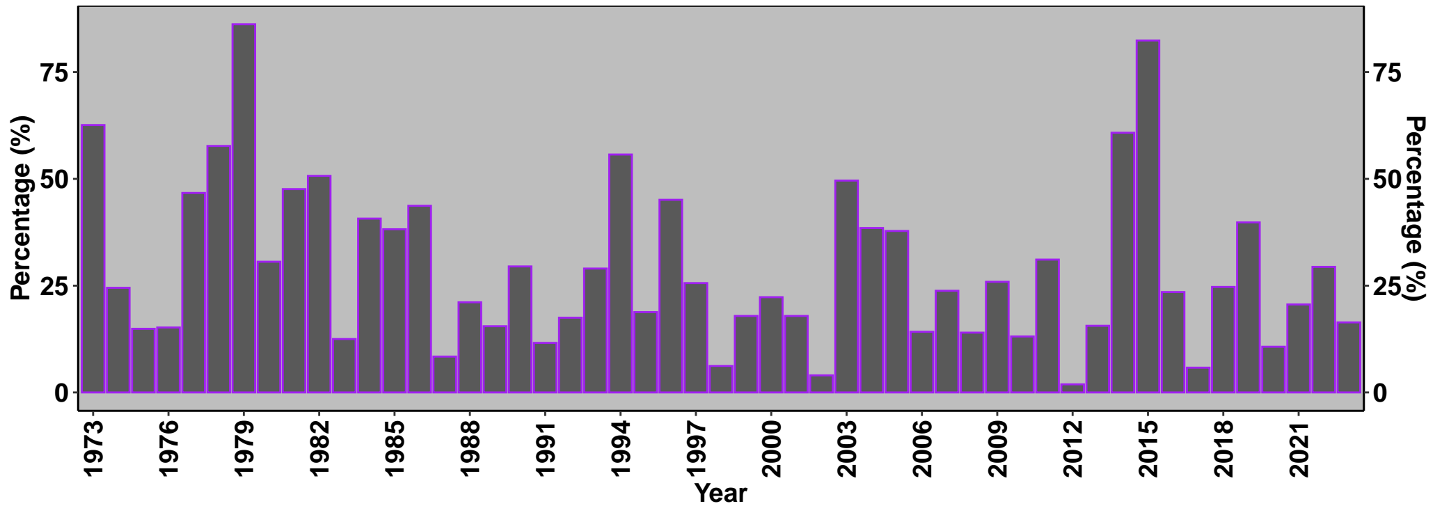
Lake Ontario Annual Maximum Ice Cover
