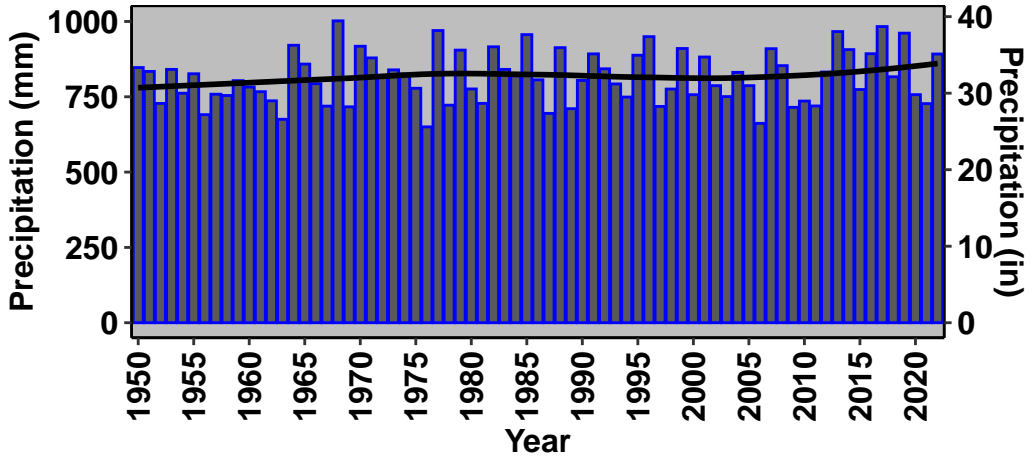
Lake Superior Annual Precipitation
