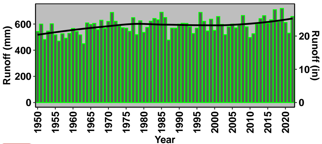
Lake Superior Annual Runoff
