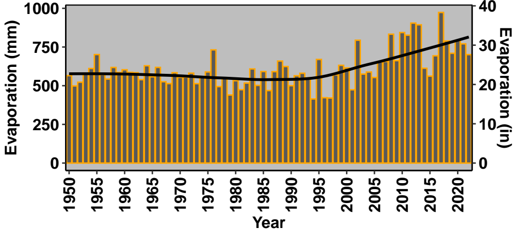
Lake Superior Annual Evaporation
