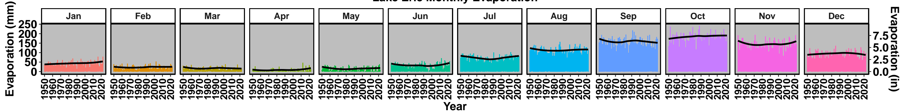
Lake Erie Monthly Evaporation
