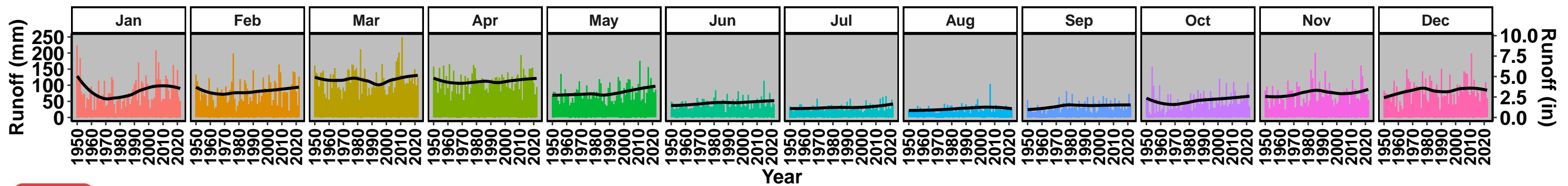
Lake Erie Monthly Runoff
