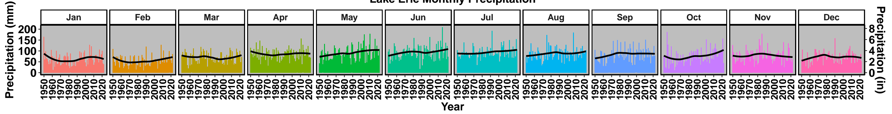
Lake Erie Monthly Precipitation
