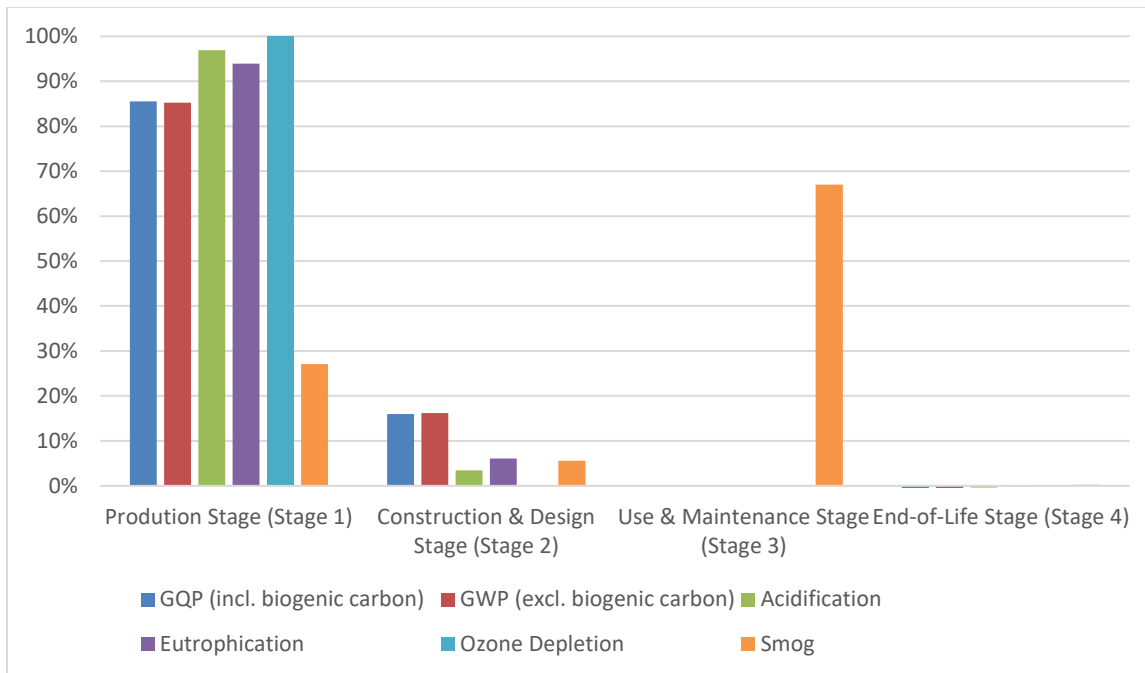
Figure 2. Impact Category Result Breakdown by ISO 21930 Stage for Average Loxon® Acrylic Block Surfacer Formulation.
