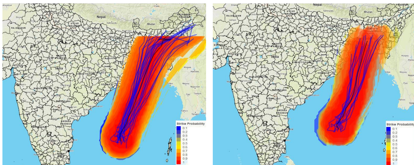
Fig. 3a: The strike probability forecasts of NEPS-G (left panel) and NEPS-R (right panel) based on 00 UTC, 18 February 2020 Super Cyclone Amphan .
