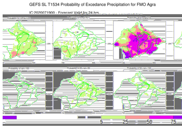
Fig.-21: GEFS based sub basin wise categorical QPF
