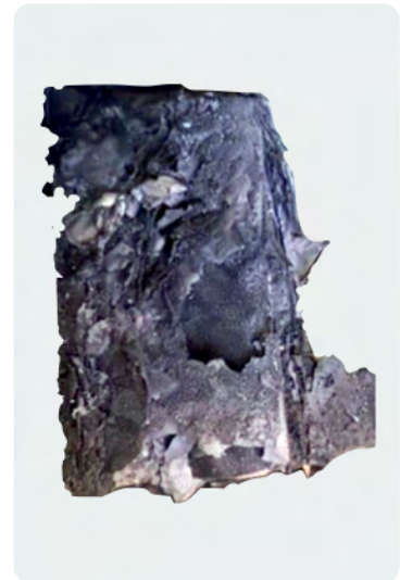
Third-party battery after an Abusive Overcharge test, which is intended to simulate charging the battery beyond its intended limits.
