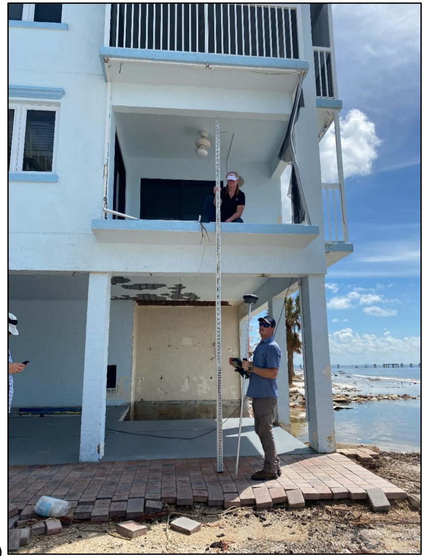
Figure 12. (a) Storm surge high water mark in bathroom cabinet on the second-story of a beachfront structure in Fort Myers Beach. (b) NWS survey team extrapolating the high water mark to the outside of the home to survey its elevation of approximately 12 ft above the brick foundation and 15 ft above MHHW. Images courtesy of the NWS.
