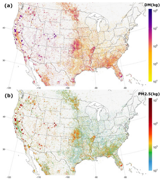
RAVE algorithm estimates of the amount of annual dry mass (DM) burned due to fires between April 2020 and March 2021 is shown in (a). The amount of fine particulate matter (PM 2.5 ) released from the fires consuming the dry mass is shown in (b). Image credit: Li, F., X. Zhang, S. Kondragunta, X. Lu, I. Csiszar, and C. C. Schmidt, Hourly biomass burning emissions product from blended geostationary and polar-orbiting satellites for air quality forecasting applications, Remote Sensing of Environment, in press, 2022.
