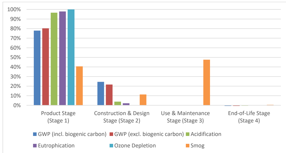
Figure 2. Impact Category Result Breakdown by ISO 21930 Stage for Average Pro Industrial™ Waterbased Alkyd Urethane Formulation.
