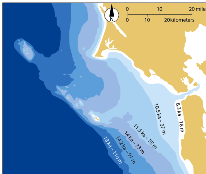
Figure 4. San Francisco Bay estuary formation. A) During glacial times, the shoreline is out beyond the Farallon Islands and a river valley occupies the site of the San Francisco Bay estuary. B) As global sea level rose since the height of the last glacial period, the shoreline gradually moved inland, passing through the Golden Gate approximately 10 thousand years ago. Adapted from Sloan, 2006 using data from Atwater 1979 and Atwater et al 1977.
