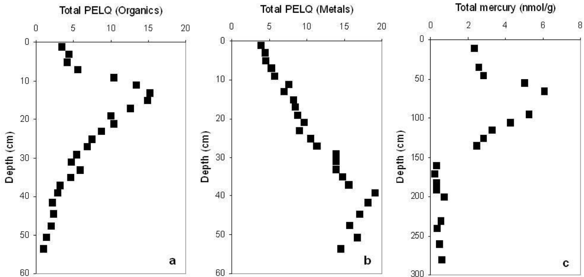
Figure 2. Depth profiles of toxicity potential of (a) organic contaminants and (b) trace metals in Stege Marsh sediment core (Hwang et al., 2008) and (c) total mercury concentrations in Triangle Marsh sediment core (Connaway et al., 2004). PELQ (Probable Effects Level Quotient) represents the degree of toxicity potential.
