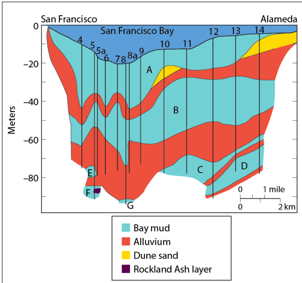
Figure 2. Sediment layers beneath the San Francisco Bay estuary between San Francisco and Alameda, the site of a proposed "southern crossing". Layer A contains the modern interglacial estuarine sediments (Bay mud), and layers B, C and D are previous interglacial estuary sediments; E, F and G may be associated with C and D. Alluvial sediments alternate between the estuary sediments, representing river-borne sediments deposited during glacial periods. Adapted, with permission, from D. Sloan, 2006.
