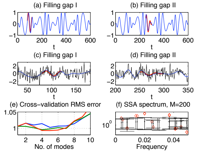
Fig. 2. Gap filling of (a, b) a nonlinear oscillatory signal s(t) , and (c, d) of its noise-contaminated version x(t) (black line) see Eq. (6), units are nondimensional. Blue line is the oscillatory component s(t) , red is the filled-in data. Gap I is over the interval 80\leq t\leq 120 , while gap II is over 250\leq t\leq 300 . (e) Cross-validation results for filling gap II in x(t) blue, green and red lines are for SSA windows of M=160, 180 and 200 , respectively. (f) Monte-Carlo SSA spectra of x(t) with window M=200 (see caption to Fig. 1).
