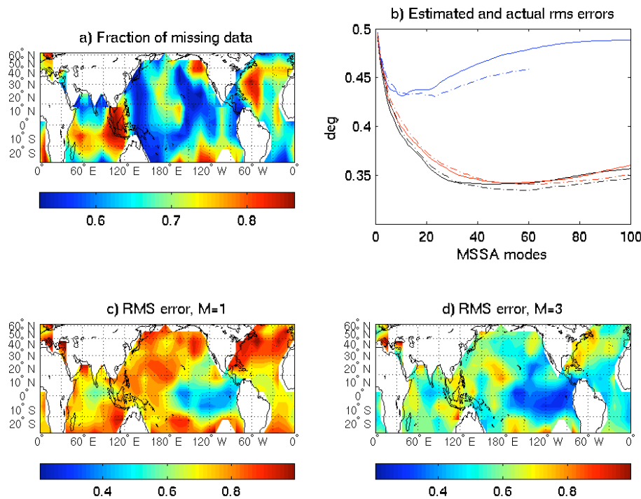
Fig. 3. Reconstruction of missing SST anomaly data for the 50-year-long monthly IRI data set. (a) Fraction of missing data (%) (b) cross-validation results for choosing optimum M-SSA window and number of modes for filling of missing data. Dashed and solid lines are the actual and estimated errors, respectively blue, black and red colors are for windows of M=1 , M=3 , and M=5 , respectively. (c, d) Root-mean-square (rms) SST error between the actual and reconstructed SST fields, computed and normalized by the standard deviation at each grid point: (c) for M-SSA window M=1 and number of modes K^*=10 (d) for optimum M-SSA window M^*=3 and K^*=50 .
