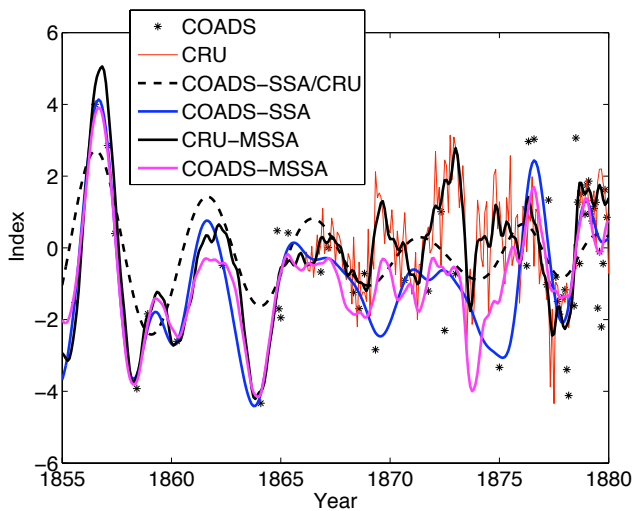
Fig. 7. Reconstruction of pre-1880 SOI time series. Different methods are applied to the COADS data set, with or without CRU data as well: original COADS data (asterisks), CRU SOI (red line) filled-in COADS: with SSA conditioned on CRU (black dashed line), with SSA of COADS data only (blue line), with M-SSA using jointly the COADS and CRU data (solid magenta) and reconstructed CRU with optimal M-SSA parameters (solid black).
