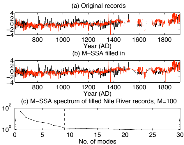
Fig. 4. Extended records (A.D. 622–1922) of low-water (solid black curve) and high-water (solid red) levels: (a) original data and (b) data with missing points filled in by M-SSA. The gap filling uses a window of M=100 yr and two channels (the low- and high-water levels). The time series have been centered on the relevant mean and the amplitudes have been normalized by the standard deviation of the original time series (excluding missing data points). The mean of the high-water record is 907 cm, while it is 288 cm for the low-water record the corresponding values for the variances are 6586 \text{ cm}^2 for the high-water record and 10\,359 \text{ cm}^2 for the low-water record. (Panels (a) and (b) reproduced from Kondrashov et al., 2005a , by permission of the American Geophysical Union). (c) M-SSA spectrum of filled Nile River records, M^*=100 years. The optimum number K^*=9 of modes corresponds to the break in the slope of the M-SSA spectrum.
