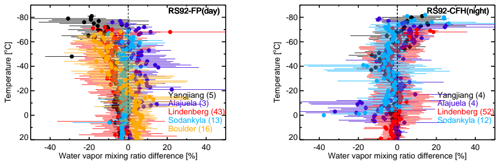
Figure 18. Comparison of humidity profiles from GRUAN-processed RS92 and coincident frost point (FP) hygrometer data. Top: daytime flights bottom: night-time flights. Data are gridded in 500 m wide bins and plotted with ambient temperature as the vertical scale. The analysis is restricted to the troposphere. The solid circles represent the relative difference \text{RS92} - \text{FP} with respect to the FP humidity, and the bars indicate the statistical uncertainty (standard deviation). All data presented here are for the CFH except for the NOAA FPH data from Boulder the number of soundings at each site is given in brackets. The approximate water volume mixing ratios at various temperature levels are given in Table 7.
