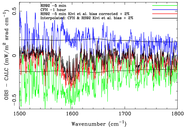
Fig. 8. Residual radiances, IASI observed minus calculated with OSS RTM, for different atmospheric profiles: CFH sonde launched 1 h before overpass (blue), RS92 sonde launched 5 min before overpass (green), same sonde but with the “Kivi et al. +2” bias correction (red) and the time interpolated profile (black) using CFH (launched 1 h before overpass) and Kivi et al. +2 bias corrected RS92 (launched 5 min before overpass) measurements. Thin black nearly flat lines correspond to three sigma IASI instrument noise.
