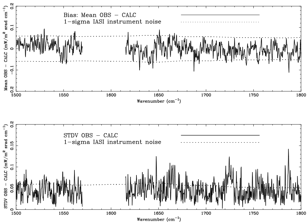
Fig. 15. Bias and standard deviation of IASI observed minus calculated radiances. The calculated radiances have been obtained using LBLRTM 11.6 and the “in situ” bias correction.
