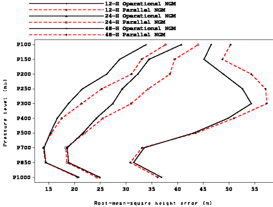
Figure 7: RMS Height error vs. rawsobs over the CONUS for the operational NGM (solid black) and the parallel NGM (dashed red) 12, 24, and 48-h forecasts from 12Z 12/16/1999 - 00Z 2/14/2000
