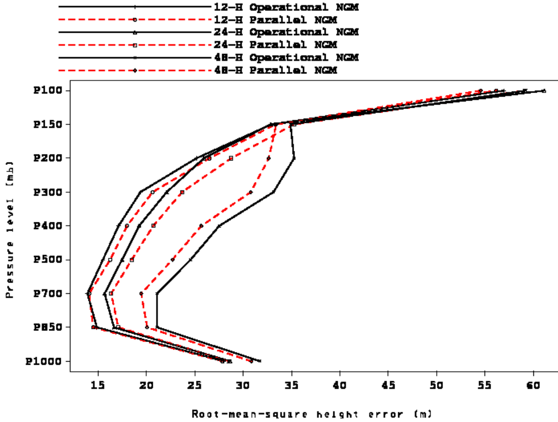
Figure 12: Same as Figure 7, but for the period 00Z 7/2/1999 - 12Z 8/2/1999
