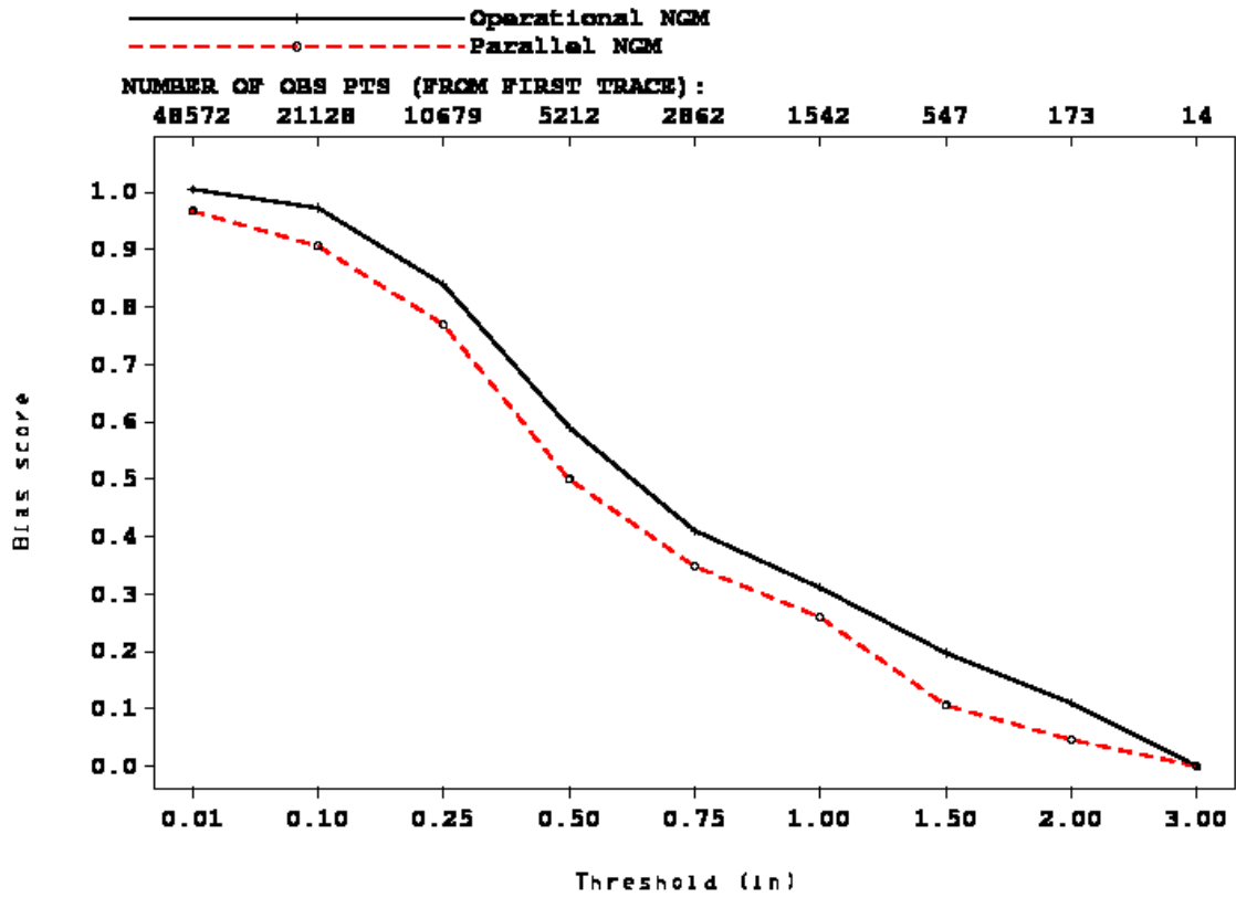
Figure 16: 24-h accumulated precipitation bias score for all operational NGM (solid black) and parallel NGM (dashed red) forecasts for the period 12Z 12/16/1999 - 00Z 2/14/2000
