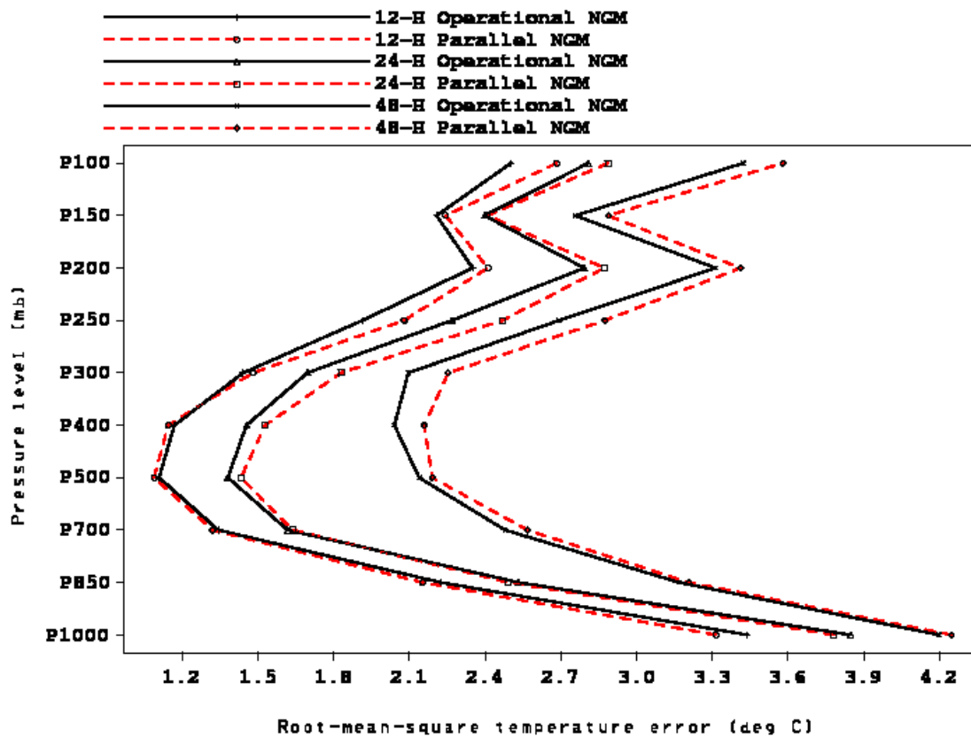
Figure 8: Same as Figure 7, but for temperatures
