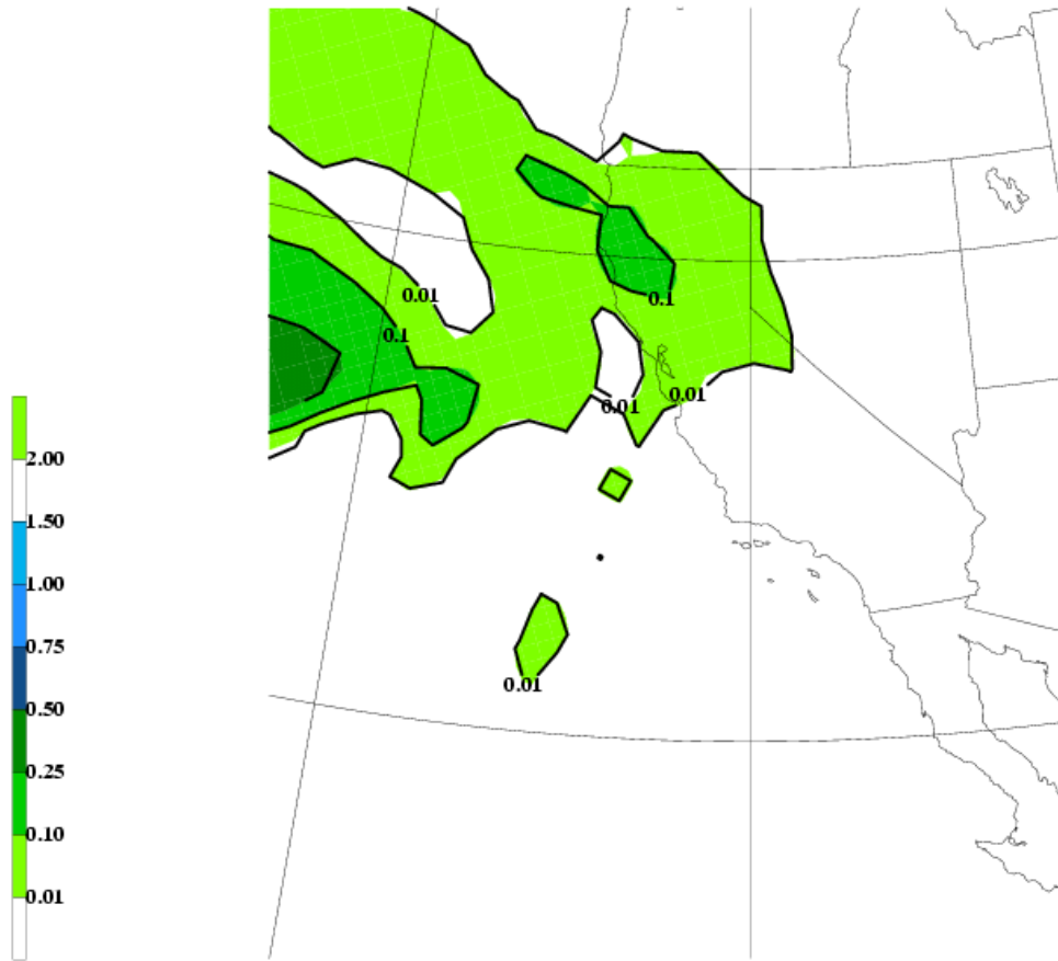
PARALLEL NGM 24-H ACCUM PRECIPITATION FORECAST VALID 12Z 2/4/2000
