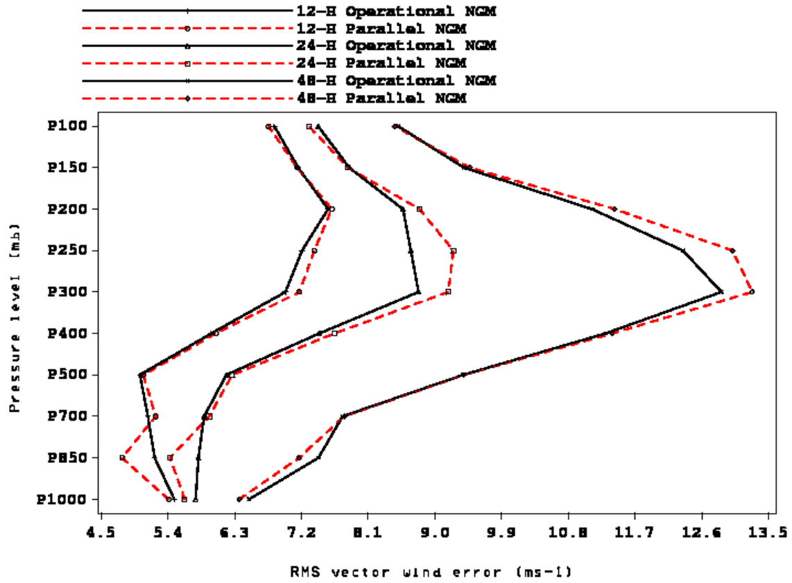
Figure 9: Same as Figure 7, but for vector wind
