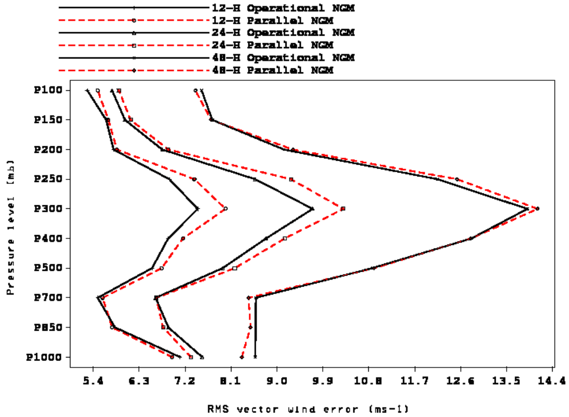
Figure 11: Same as Figure 9, but over Alaska
