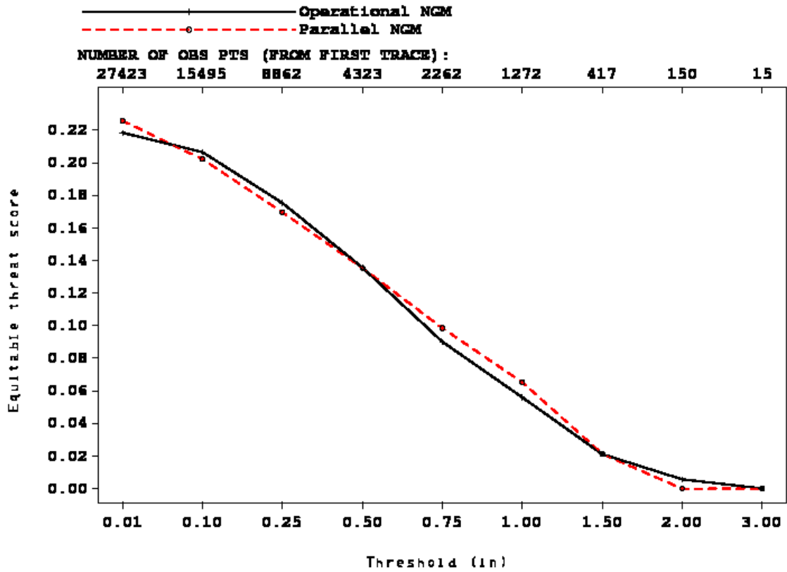
Figure 24: Same as Figure 17, but for the period 00Z 7/2/1999 - 12Z 8/2/1999
