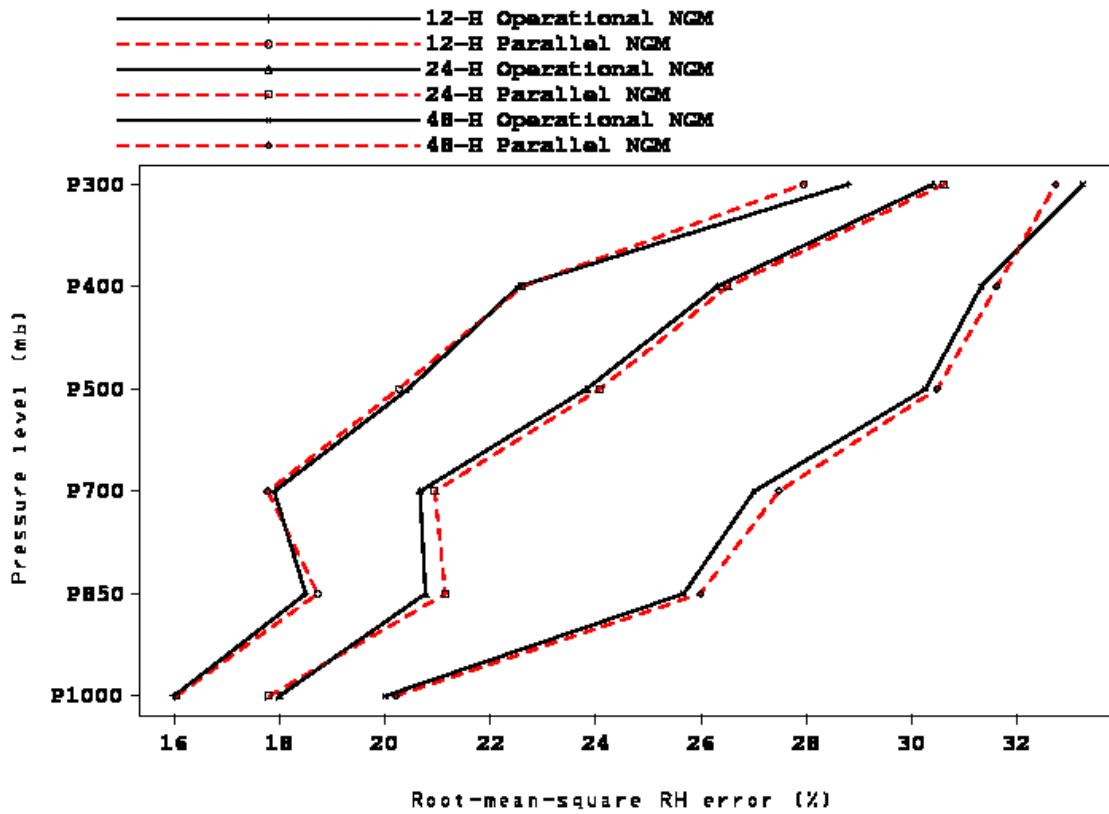
Figure 10: Same as Figure 7, but for relative humidity
