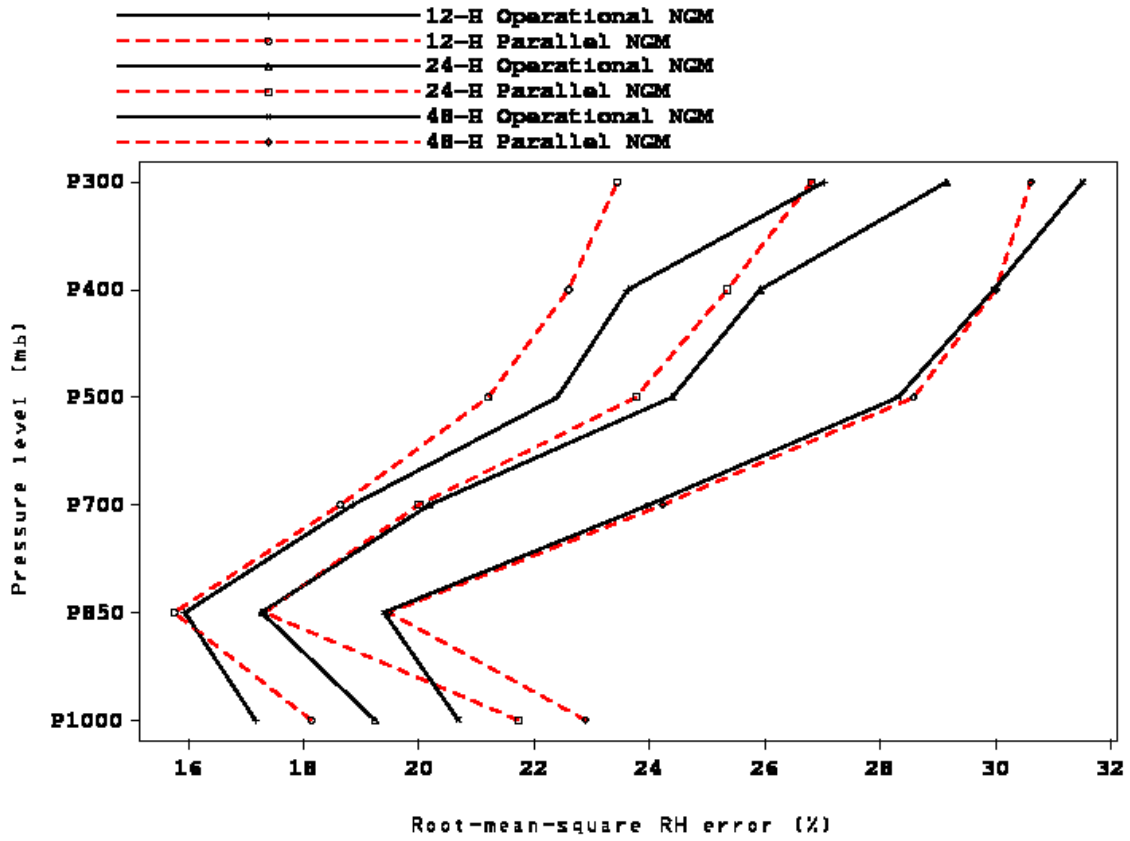
Figure 15: Same as Figure 10, but for the period 00Z 7/2/1999 - 12Z 8/2/1999
