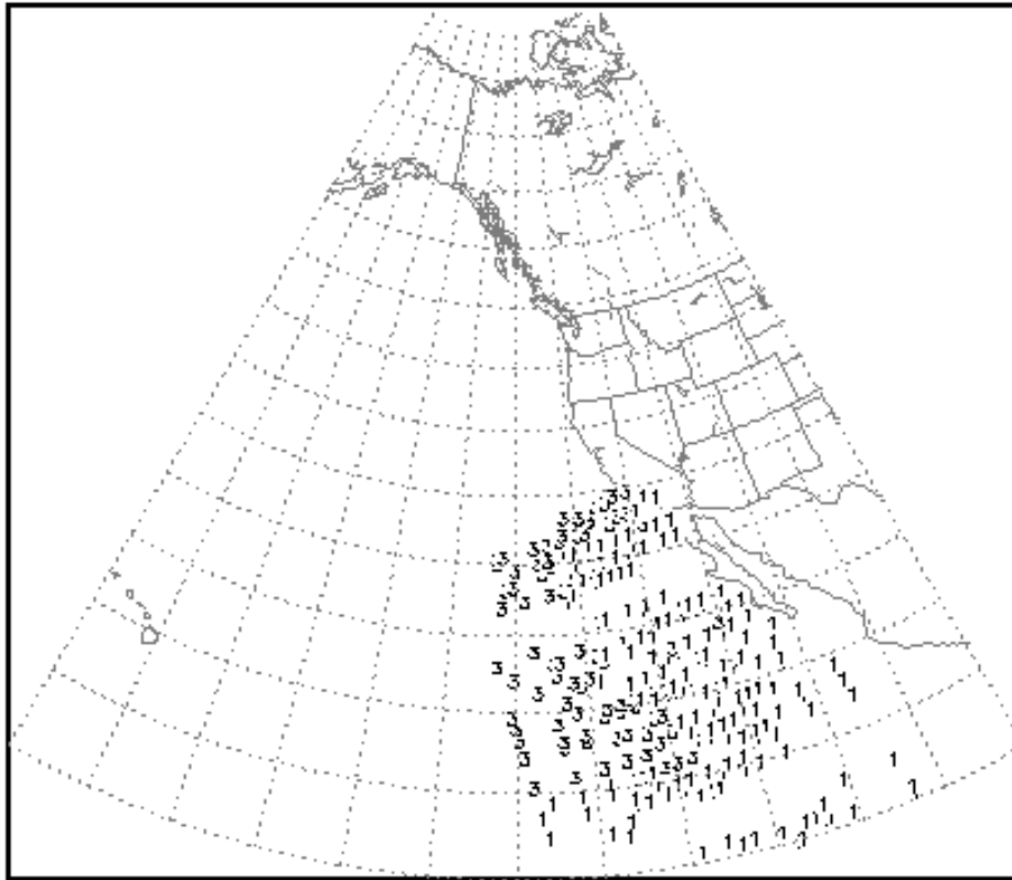
Figure 3: Locations of satellite temperature observations used by the 00Z 2/14/2000 Eta analysis
