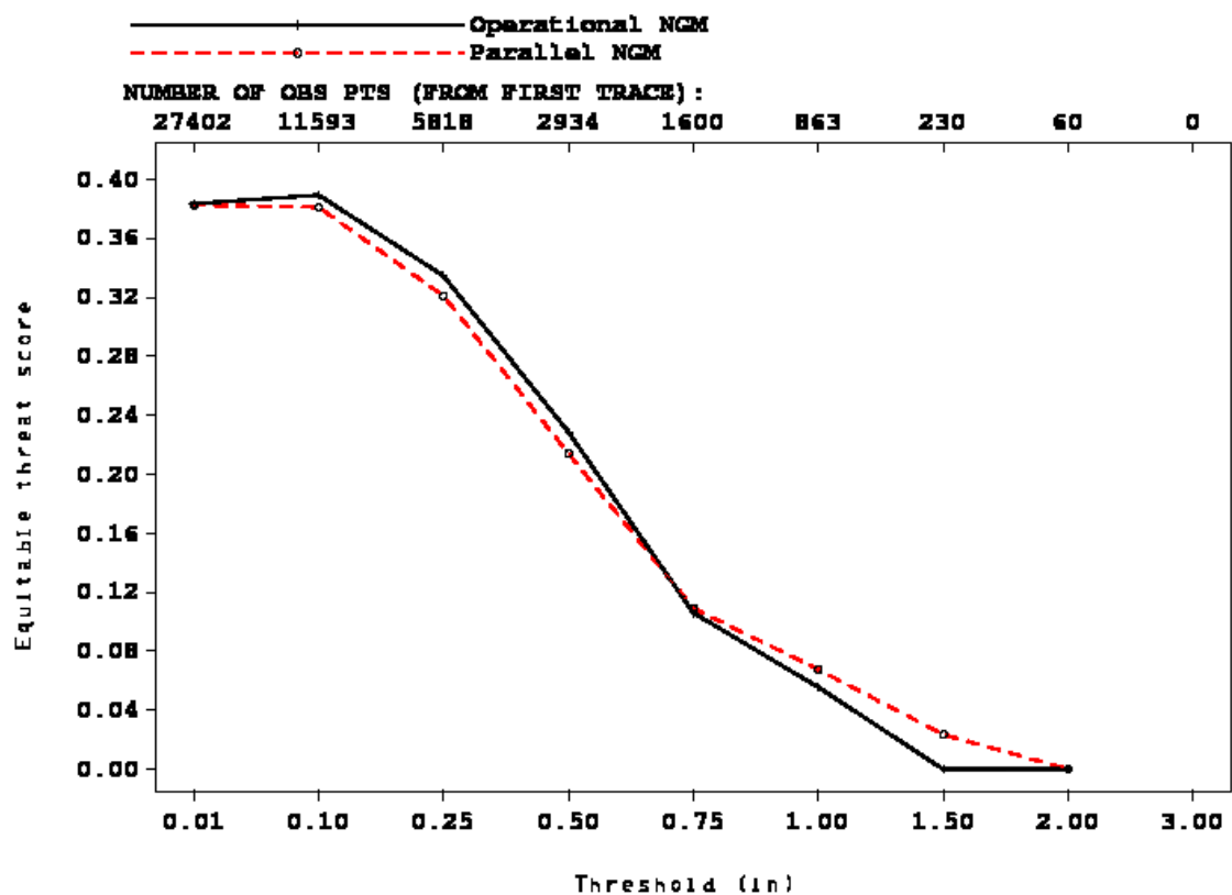
Figure 19: Same as Figure 17 but for the eastern U.S. (area defined in Figure 18)
