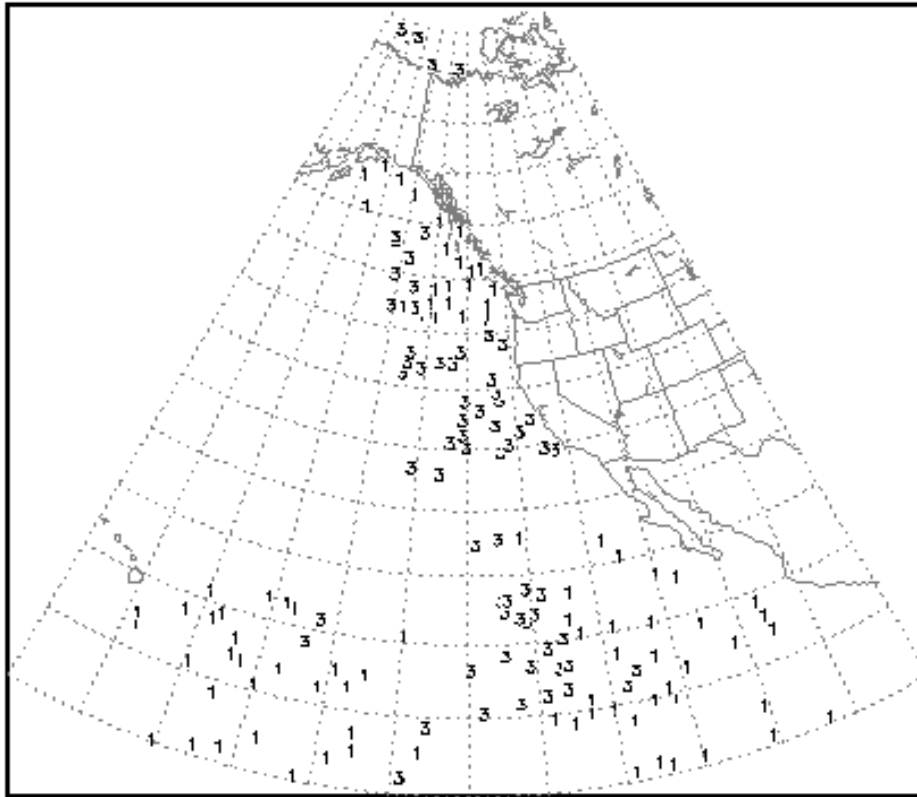
Figure 4: Locations of satellite temperature observations used by the 00Z 2/14/2000 RAFS analysis
