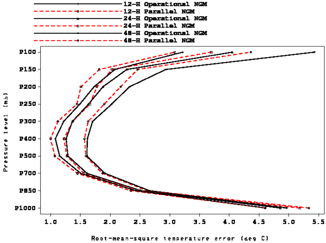
Figure 13: Same as Figure 8, but for the period 00Z 7/2/1999 - 12Z 8/2/1999
