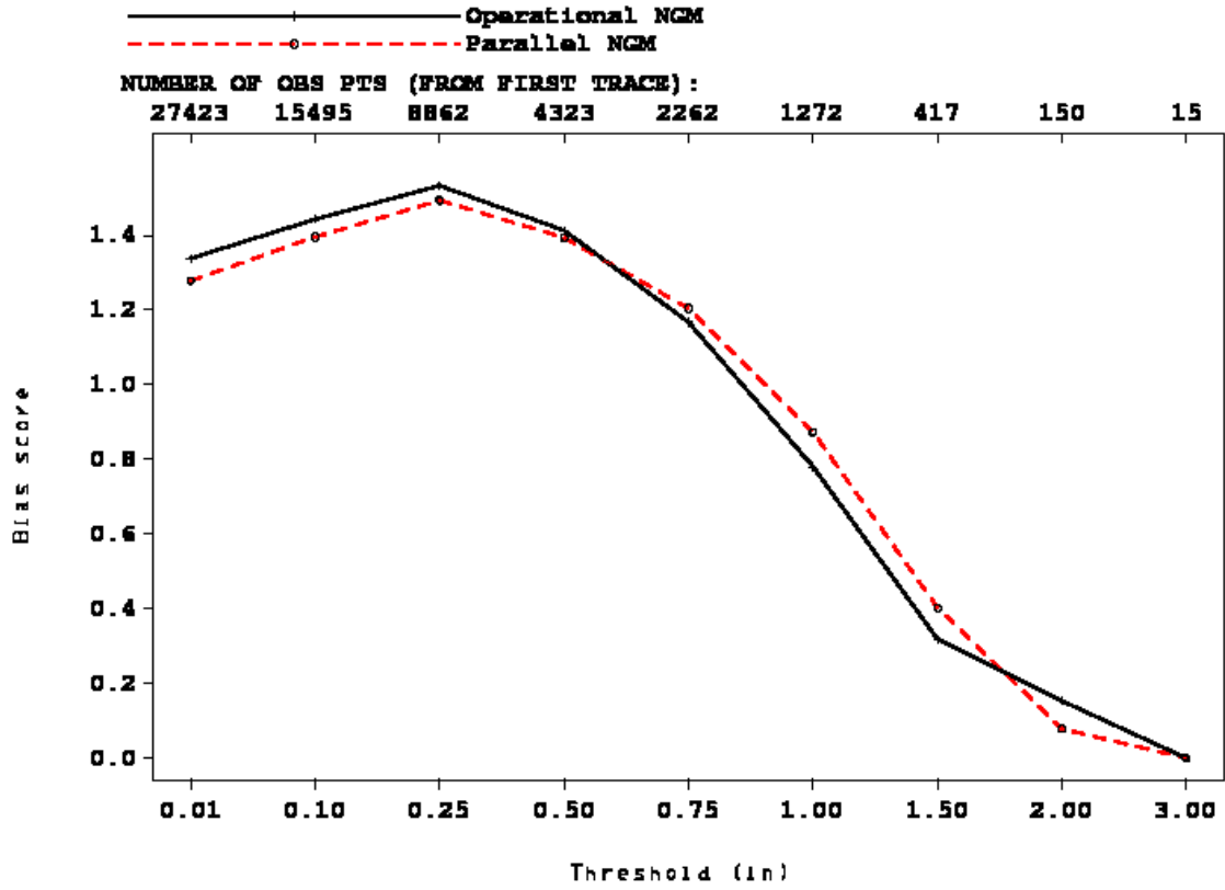
Figure 23: Same as Figure 16, but for the period 00Z 7/2/1999 - 12Z 8/2/1999
