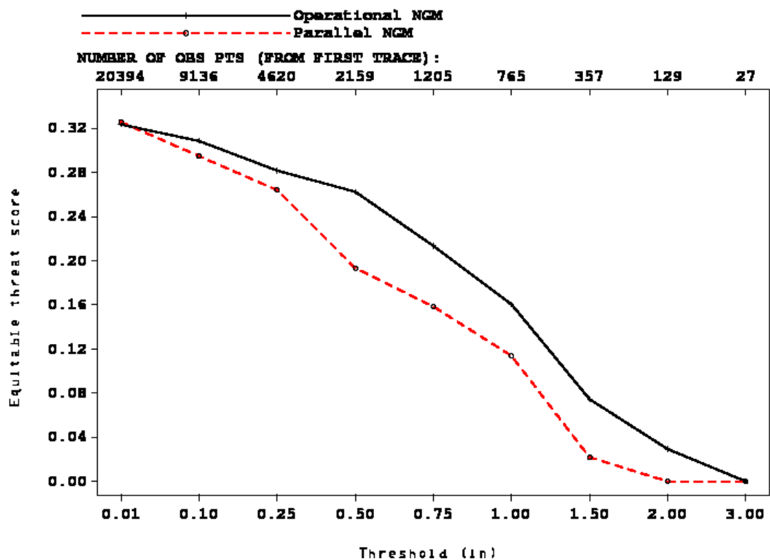
Figure 20: Same as Figure 17 but for the western U.S. (area defined in Figure 18)
