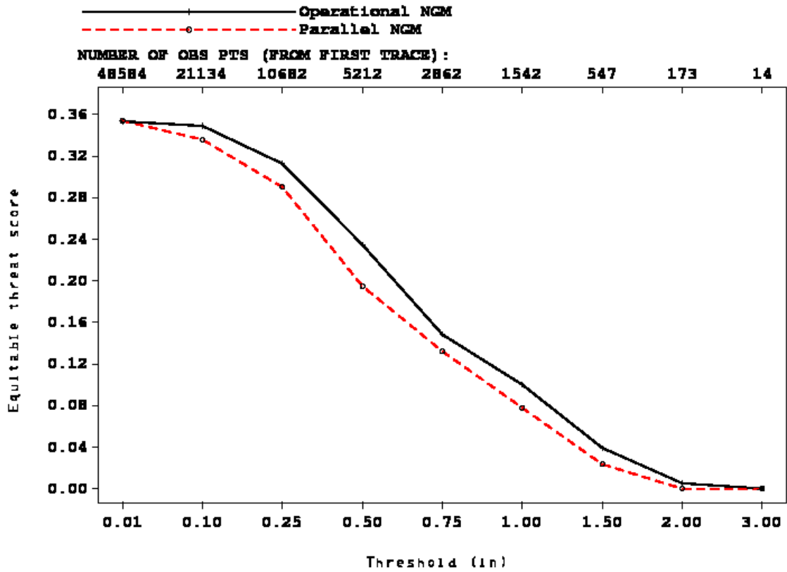
Figure 17: Same as Figure 16 but for 24-h accumulated precipitation equitable threat score
