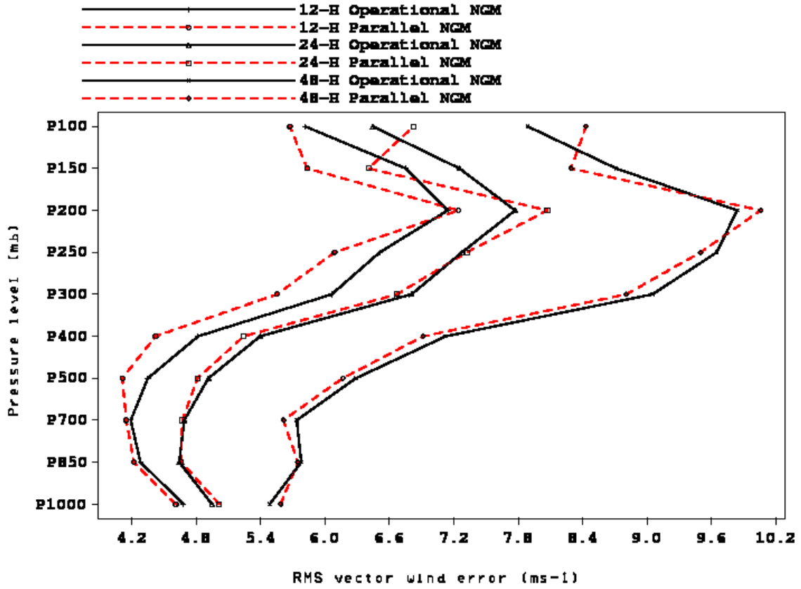
Figure 14: Same as Figure 9, but for the period 00Z 7/2/1999 - 12Z 8/2/1999
