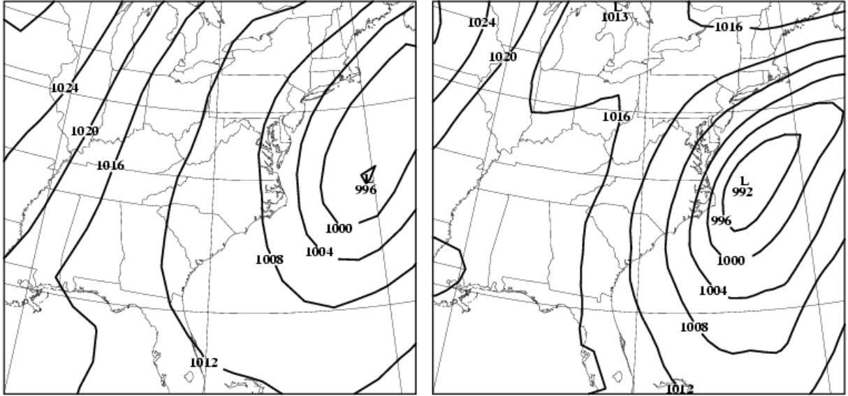
OPERATIONAL NGM 24-H FCST
