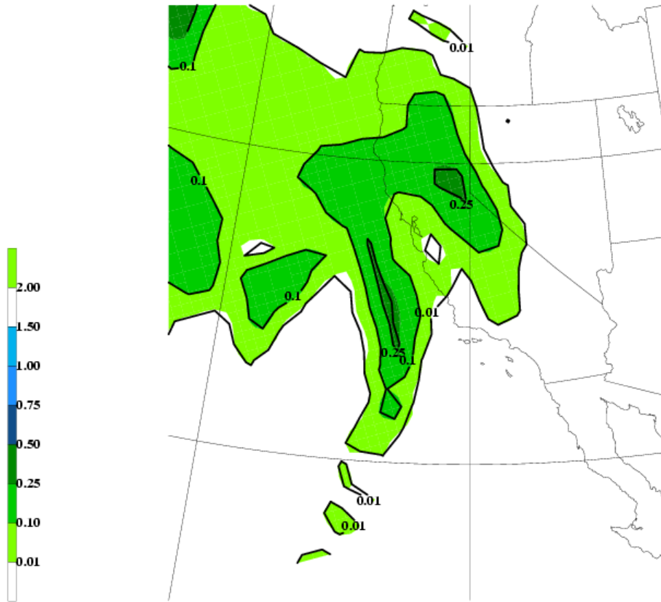
OPERATIONAL NGM 24-H ACCUM PRECIPITATION FORECAST VALID 12Z 2/4/2000
