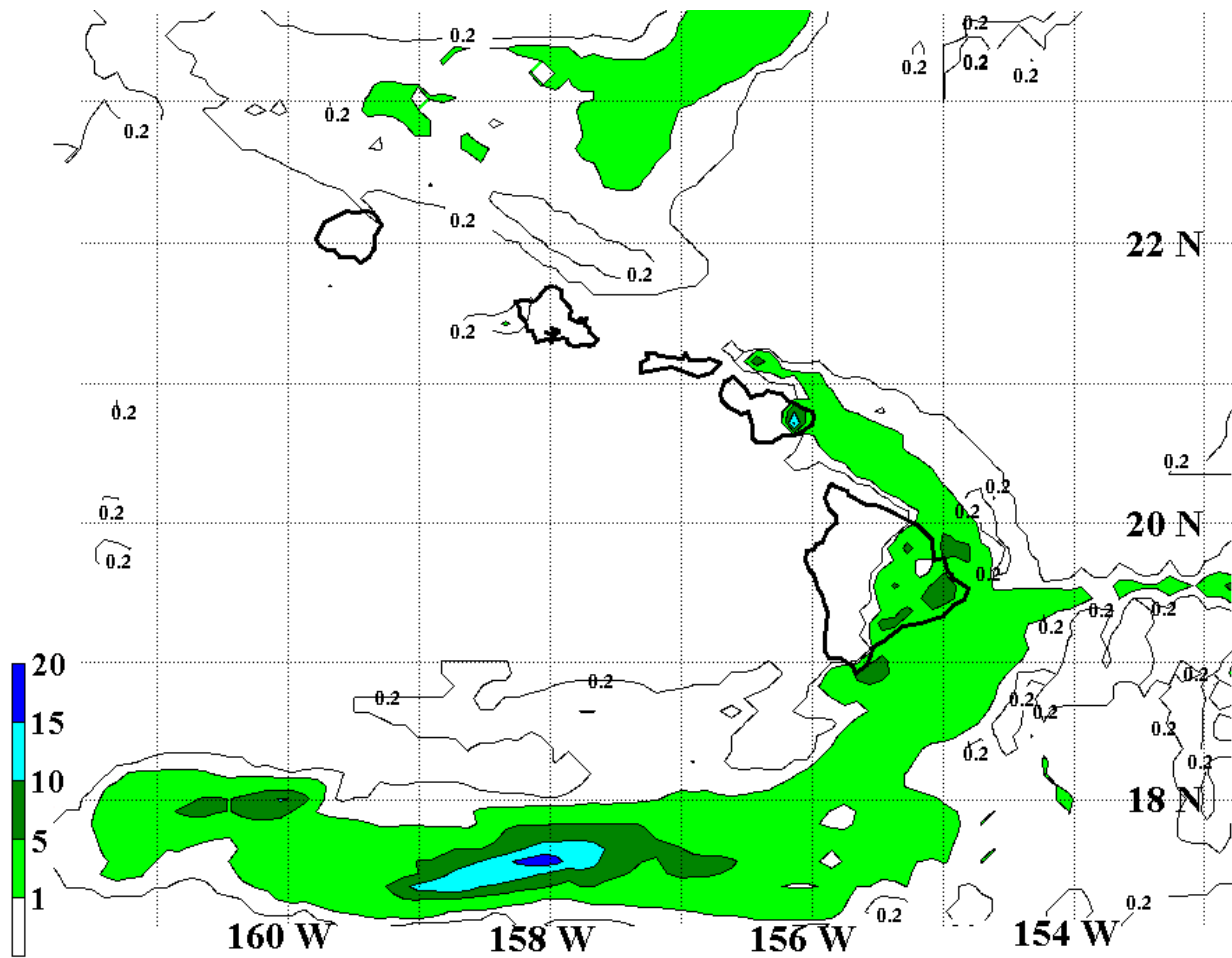
RSM 24-h accumulated rainfall (mm), 1800 UTC 28 April to 1800 UTC 29 April 1997
