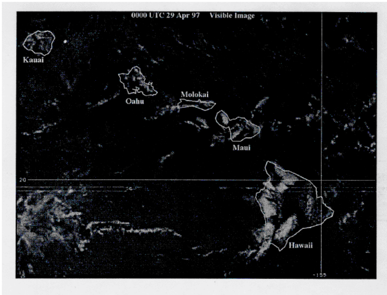
Fig. 6. GOES-9 visible wavelength image for 0000 UTC 29 April 1997.
