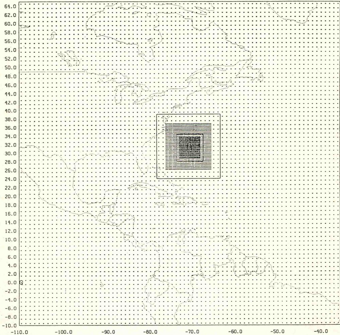
Figure 1. Grid points and model domain for the triply-nested GHM forecast initiated on 0000 UTC 30 August with the inner two grids centered on Hurricane Emily (1993).
