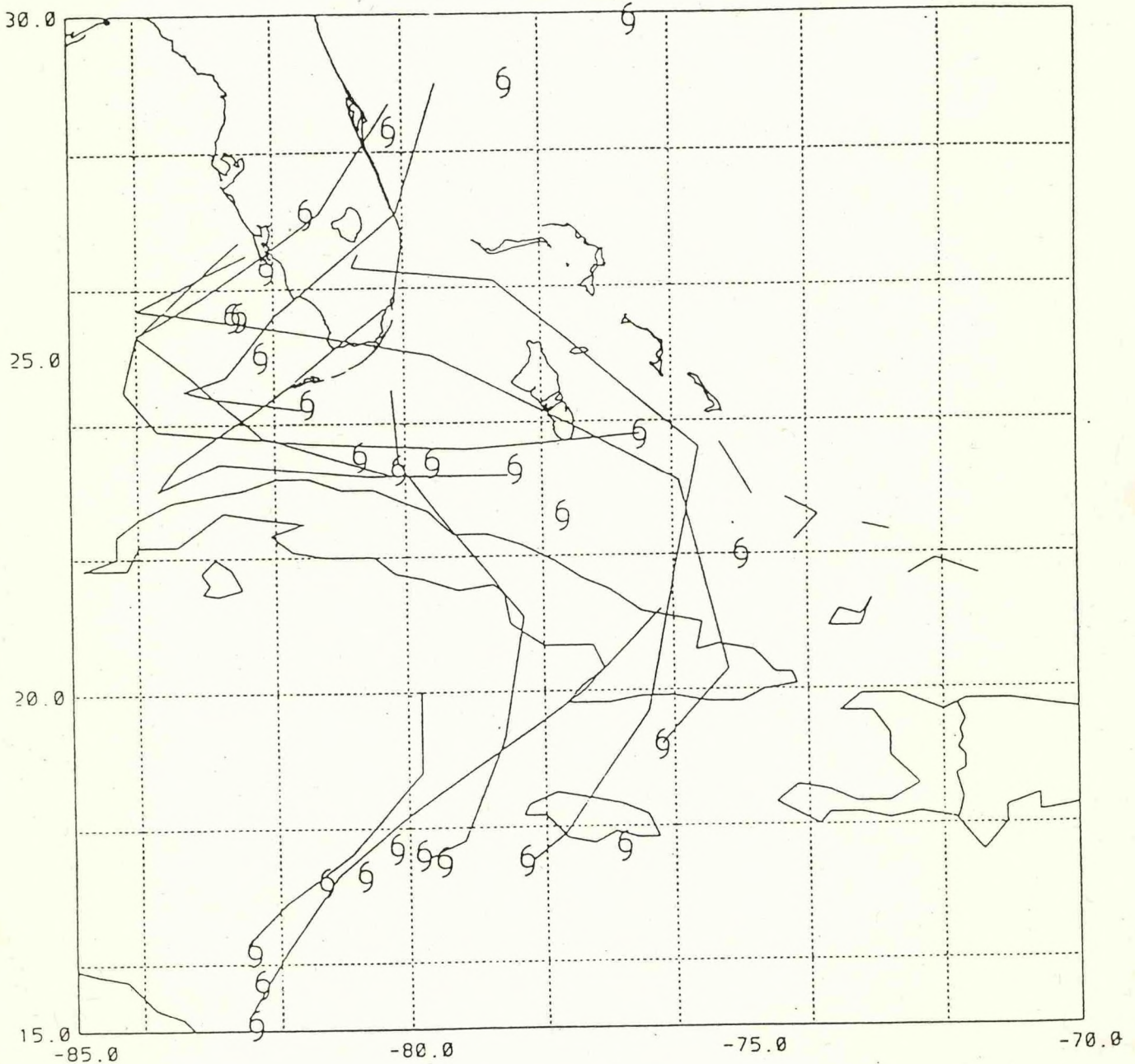
Figure 5. Composite of track forecasts for Hurricane Gordon. Only the forecasts made prior to landfall over Florida are shown. Also plotted are the observed positions every 6 hours from 0000 UTC 11 Nov. to 1200 UTC 17 Nov. 1994.
