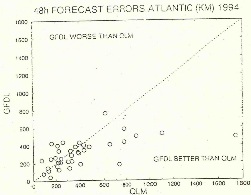
Figure 7. Forecast track errors (km) at 48 hours for all cases in the East Pacific (top) and the Atlantic (bottom) for the GHM compared to the QLM model. All circles below the dotted line indicate forecasts in which the GHM forecast errors were less than the QLM. All circle above the line indicate forecasts in which the QLM errors were less than the GHM.
