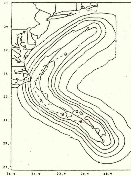
Figure 4. Distribution of maximum surface wind during the passage of Hurricane Emily for four forecasts (29 & 30 Aug., 0000 & 1200 UTC) of the GHM. Solid and dashed lines indicate forecast and observed tracks respectively. Isopleths are in knots.
