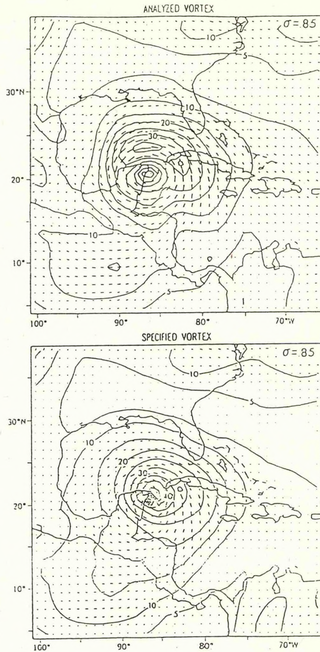
Figure 3. Distribution of horizontal wind vectors and wind speed ( \text{m s}^{-1} ) at 1200 UTC 14 September 1988 (Hurricane Gilbert) at model level 14 ( \sigma = .856 ), for both the global analysis (top) and the specified vortex (bottom). The region shown is for a portion of the integration domain surrounding the storm region. The wind distribution shown, plotted with a 5\text{-m s}^{-1} contour interval, is for the wind field resolved by the 1^\circ resolution.
