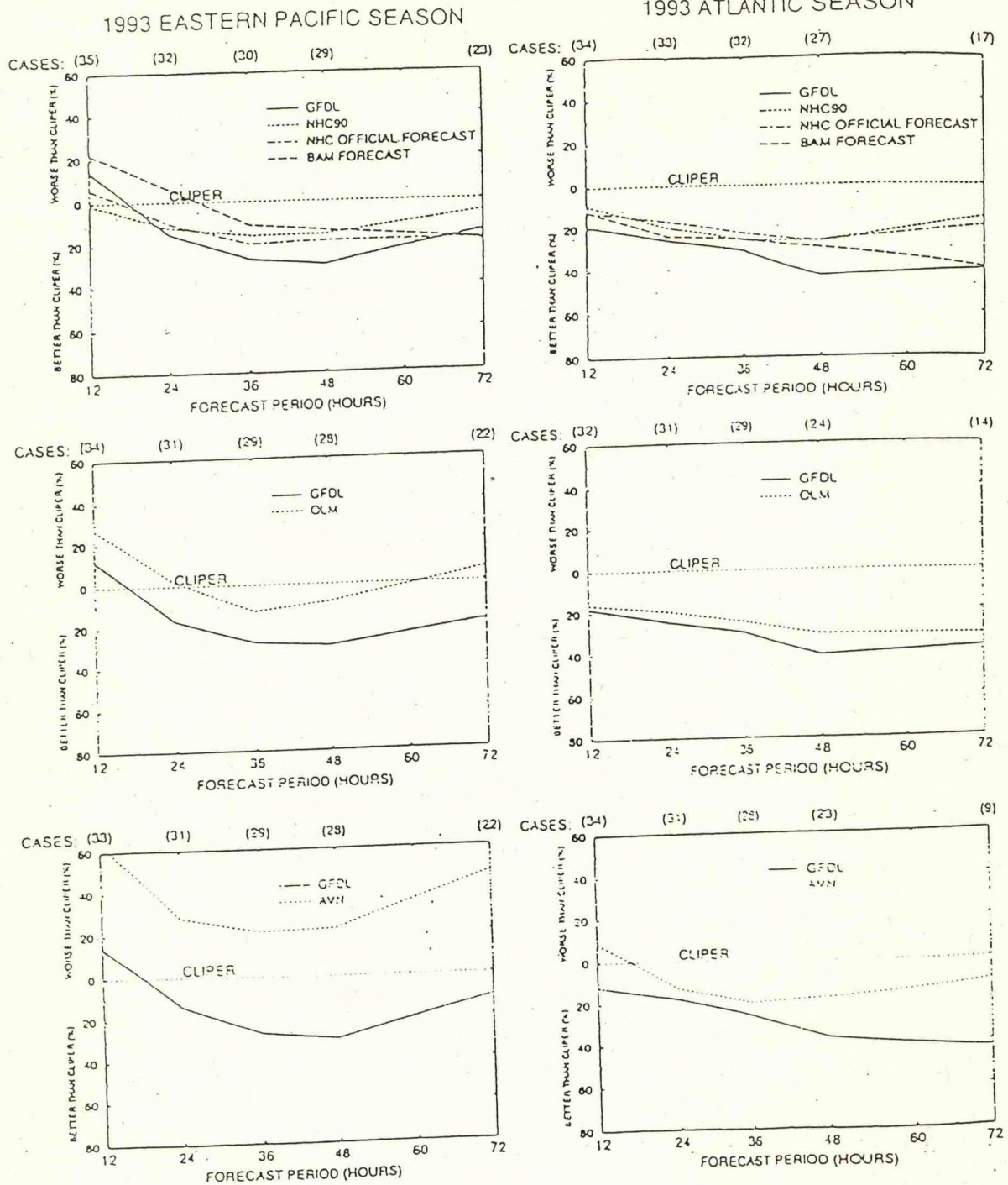
Figure 9. Summary of GHM track errors relative to Cliper for the Eastern Pacific (left) and Atlantic (right) for the 12- to 72-h forecast period. GHM results are indicated by solid lines whereas other model forecasts are indicated by dotted or dashed lines. Forecast error percentages indicate skill relative to climatology and persistence.
