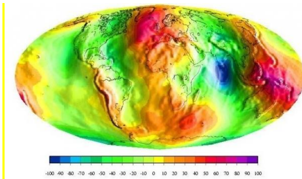
Figure 13 : EGM2008 geoid
