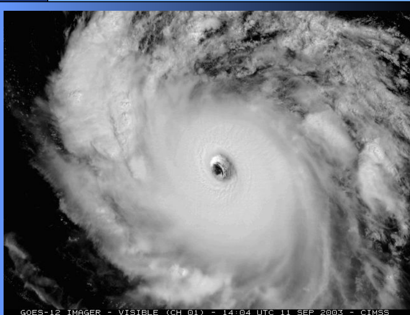
GOES-12 IMAGER - VISIBLE (CH 01) - 14:04 UTC 11 SEP 2003 - CIMSS
