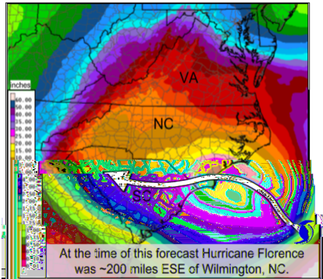
5-day Rainfall Forecast - Issued Sep 13, 2018
