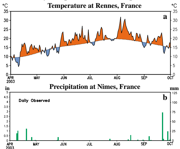
Fig. 2. Daily mean (a) surface temperatures (°C) at Rennes, France and (b) precipitation at Nimes, France. Temperature anomalies in (a) are shaded, with red indicating above-average temperatures. Scale for precipitation is inches (on the left) and mm (on the right).
