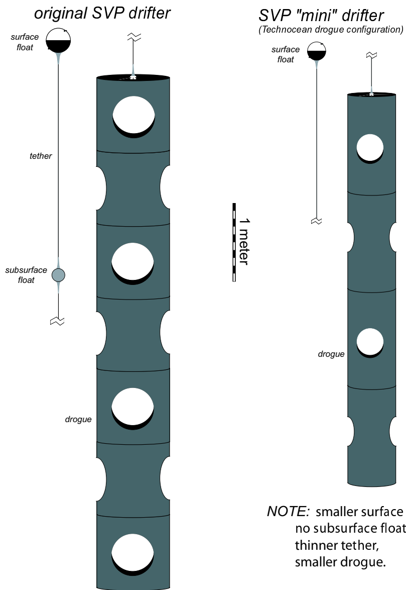
Figure 1: Schematic view of two SVP drifter types. All components are shown to scale; much of the tether length has been excluded. The drogues are centered at a depth of 15m.
