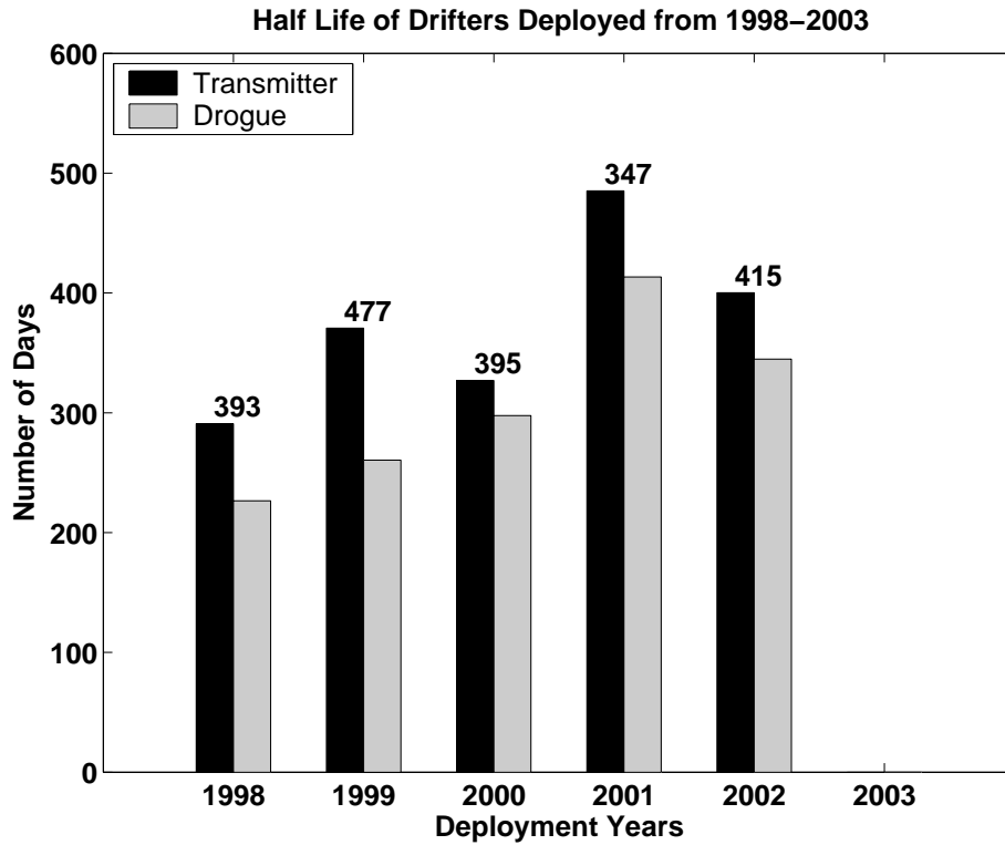
Figure 2: Half lives (days) of drifters deployed in 1998–2003. Black bar: half life of transmitter (e.g., velocity observations). Light grey bar: half life of drogued position observations. Numbers above the bars indicate how many drifters went into each calculation, e.g. how many drifters were deployed that year which did not run aground or were picked up. The 2003 half lives could not be determined because more than half are still alive and drogued.
