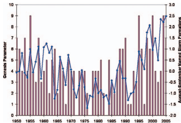
FIG. 4. The GP and Aug–Sep named storm formations south of 25°N for 1950–2005—GP is the blue solid line, and named storm formations south of 25°N are the red columns. Note that, in general, more named storm formations occur when GP values are above average.
