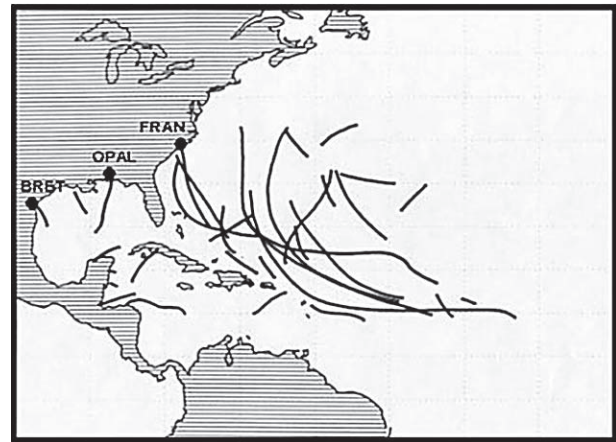
FIG. 2. Atlantic basin major hurricane tracks for the 1995–2003 seasons.
