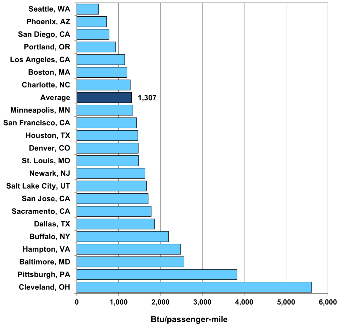
Figure 7.3. Energy Intensity of Light Rail Transit Systems a , 2019
