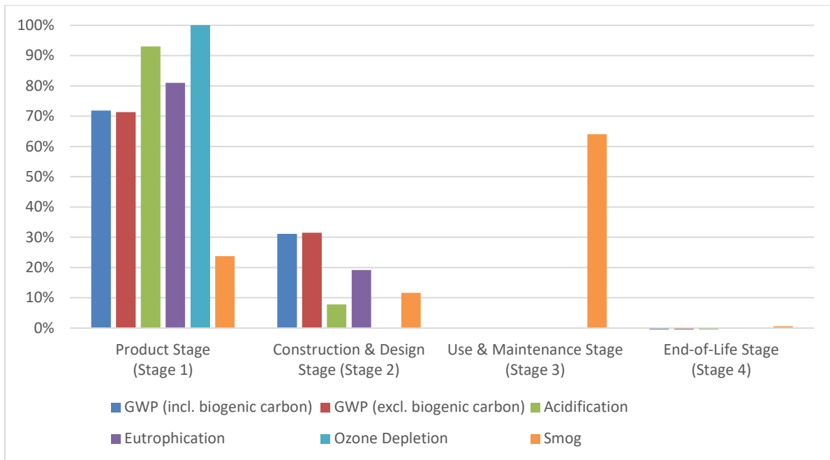
Figure 2. Impact Category Result Breakdown by ISO 21930 Stage for Average Extreme Bond™ Int/Ext Bonding Primer Formulation.
