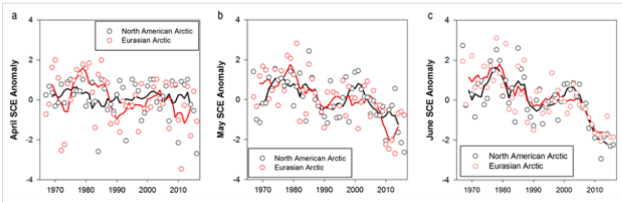
Fig. 2.1. Monthly snow cover extent (SCE) for Arctic land areas (>60° N) from the NOAA snow chart Climate Data Record (CDR) for (a, left) April (b, center) May and (c, right) June from 1967 to 2016. Anomalies are relative to the average for 1981-2010 and standardized (each observation differenced from the mean and divided by the standard deviation and thus unitless). Solid black and red lines depict 5-yr running means for North America and Eurasia, respectively.
