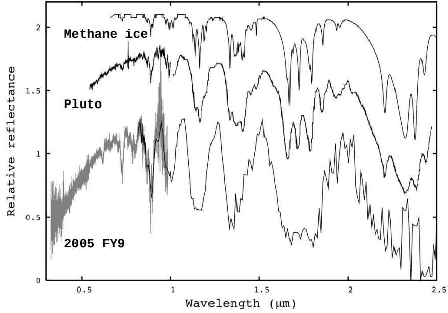
Fig. 1. Reflectance spectra of laboratory methane ice, Pluto (Grundy & Fink, 1996), and 2005 FY 9 . Spectra are normalized at 0.6 \mu m and vertically shifted for clarity. Pluto and 2005 FY 9 show very similar chemical surface composition. Figure from Licandro et al. (2006).
