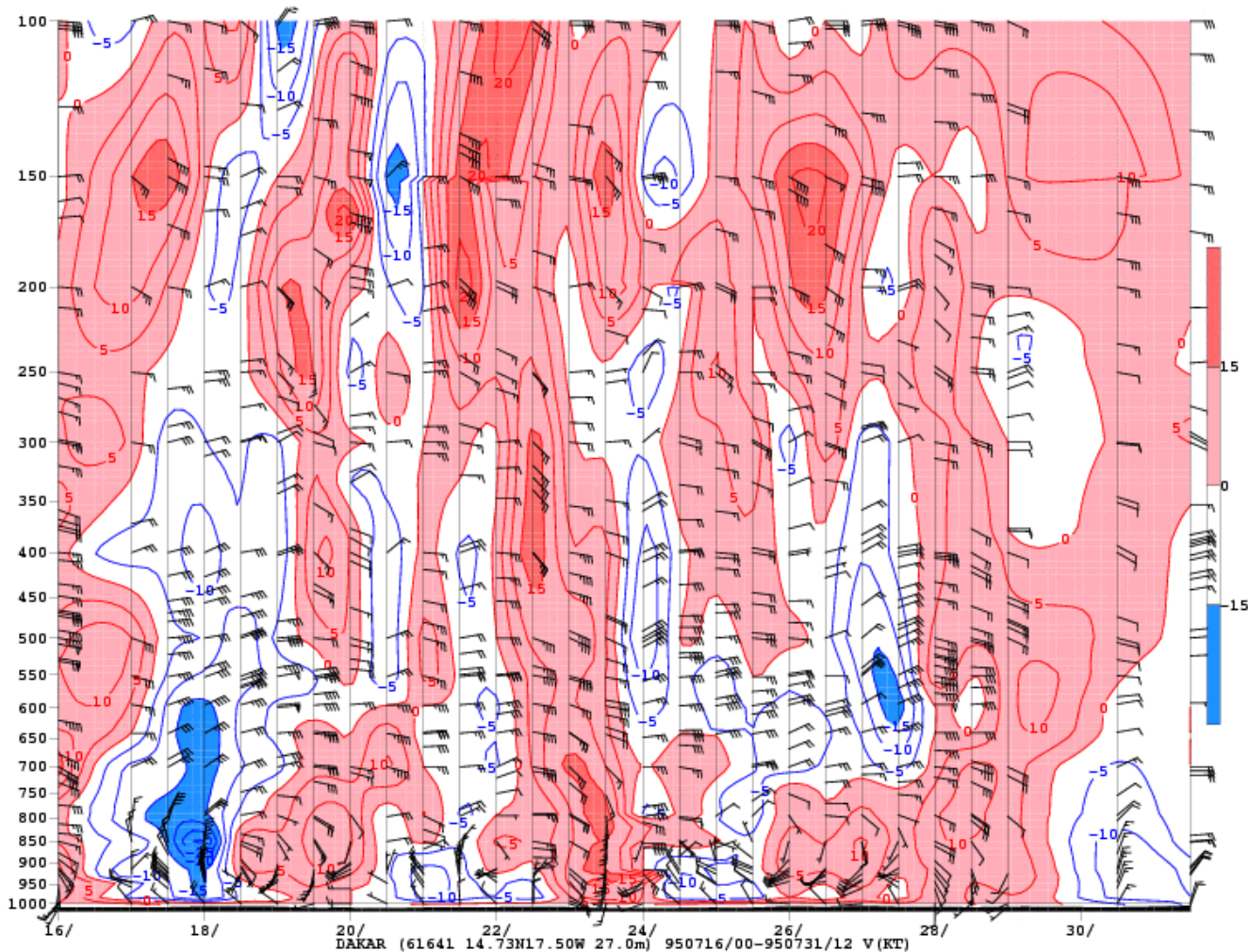
Figure 3. An example from mid-July 1995, showing a trio of waves emerging off the coast of west Africa.
