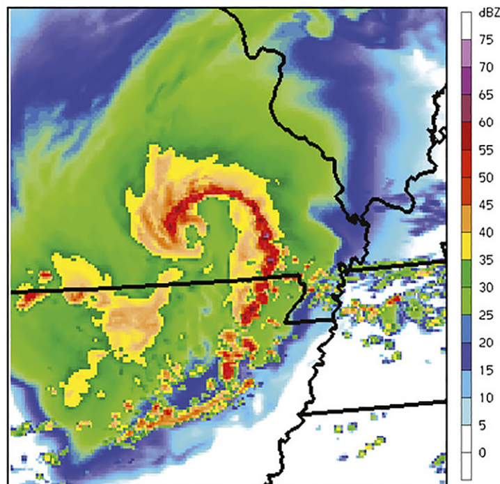
Fig. 9. (a) Paducah, Kentucky (PAH), Weather Surveillance Radar-1988 Doppler (WSR-88D) level II 0.5^\circ radar reflectivity (dBZ) at 1756 UTC 8 May 2009. (b) Column maximum derived reflectivity (dBZ) from 27 h 3 km WRF-ARW real-time forecast, valid at 1545 UTC 8 May 2009. [From Weisman et al. (2013, Fig. 1).]
