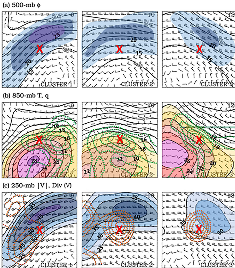
Fig. 14. A composite plot of multiple warm-season DMCS environments driven by upper ridging, showing (a) the mean 500 hPa geopotential height ( \phi ; contours every 60 m), wind (flag: 50 kt or 25 \text{m s}^{-1} ; full barb: 10 kt or 5 \text{m s}^{-1} ), and wind speed ( |V| ; shaded every 5 \text{m s}^{-1} , starting at 15 \text{m s}^{-1} ) for three clusters within the upper-ridging pattern. (b) As in (a), but for the 850 hPa temperature ( T ; solid contours every 2°C, with shading for values over 16°C) and specific humidity ( q ; green dashed contours every 1 \text{g kg}^{-1} starting at 8 \text{g kg}^{-1} ). (c) As in (a), but for the 250 hPa wind speed ( |V| ; shaded every 5 \text{m s}^{-1} , starting at 25 \text{m s}^{-1} ); divergence of the wind \text{Div}(V) ; orange dashed contours every 0.25 \times 10^{-5} \text{ s}^{-1} ). The horizontal and vertical dimensions of each grid are 2600 km and 2400 km, respectively. The "X" symbol denotes the mean position of the DMCS at the analysis time. The number of cases comprising a cluster for each synoptic pattern (left) 9, (center) 10, and (right) 12. [Subjectively augmented from Coniglio et al. (2004, Fig. 7).]
