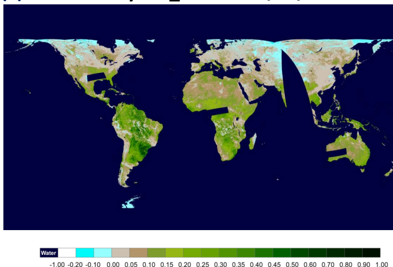
(a) Global Daily EVI_TOC on 01/04/2018
