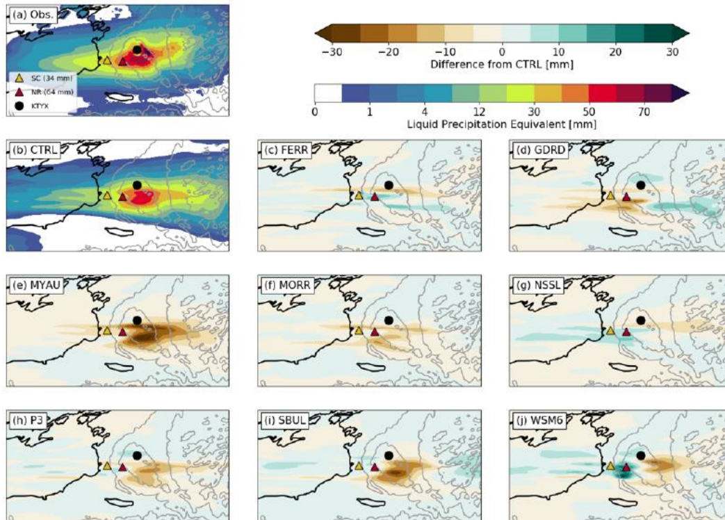
Figure 4. Observed and WRF-simulated 24-h accumulated precipitation ending at 0000 UTC 12 December 2013. (a) Precipitation measured by OWLeS manual observations (filled triangles) and estimated by KTYX radar (shading). (b) WRF quantitative precipitation forecast (QPF) over the same 24-h period for HRRR-like control member (CTRL). (c)-(j) QPE differences, relative to CTRL for remaining MP ensemble members. Taken from Bartolini (2019).
