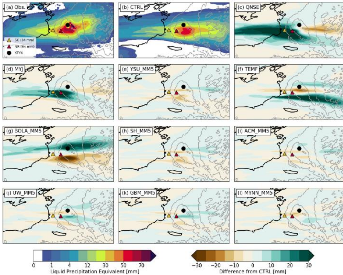
Figure 5. As for Figure 4, but for PBL/SL experiment suite. Taken from Bartolini (2019).
