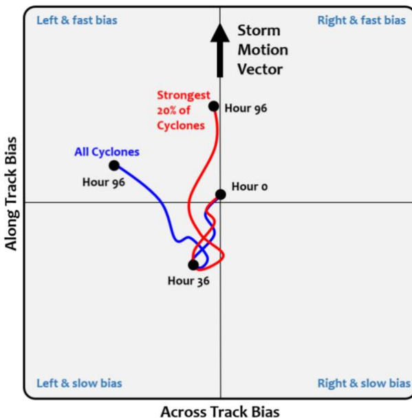
Figure 7. A schematic representation of the along-track and across-track biases for all 517 Northeastern cyclones (blue) and the strongest 20% of cyclones (red) at GEFSRv2 forecast lead-time from 0 to 96 hours.
