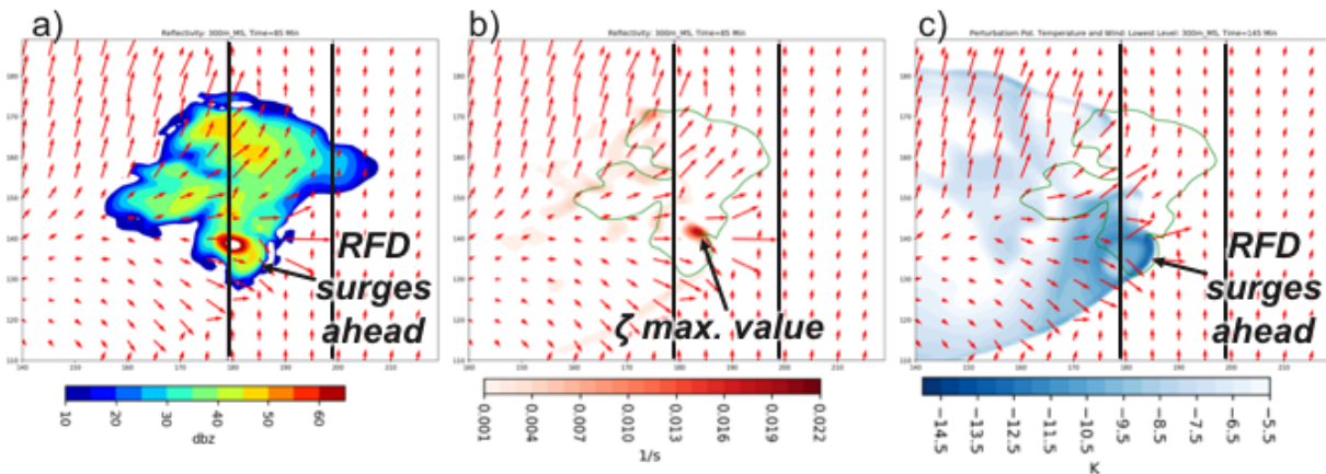
Figure 3. (a) Simulated reflectivity (dBZ), (b) 1-km relative vorticity ( s^{-1} ), (c) perturbation potential temperature (K). Red arrows are near-surface wind. Black lines denote the edges of the valley. As the rear-flank downdraft surges ahead, the low-level mesocyclone occludes and the supercell transforms into a bow echo. In contrast, a control simulation without the valley has a quasi-steady supercell through the whole simulation (not shown).
