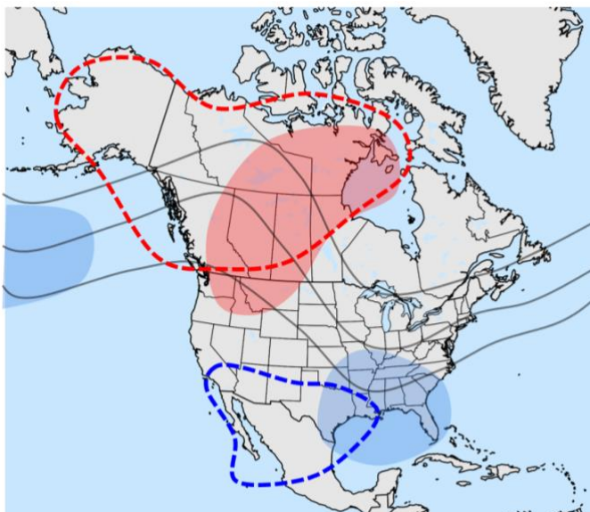
Figure 9. Composite of the 500-hPa geopotential height (black) in the subset of cases with small across-track variability. The positive and negative 500-hPa height anomalies associated with small across-track variability are shaded red and blue, respectively. The locations where the 500-hPa geopotential heights are higher or lower for small across-track bias cases compared to large-across track bias cases are within the red and blue dashed regions, respectively.
