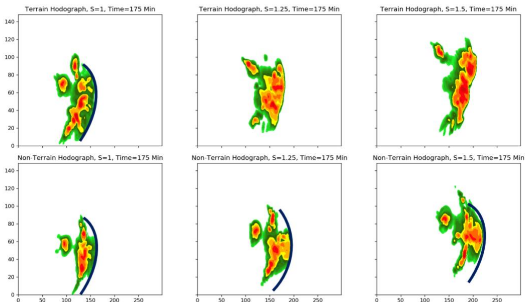
Figure 1. Simulated radar reflectivity for high-CAPE, low- (first column), medium- (second column), and high- (third column) shear simulations. The top (bottom) row of simulations has a low-level wind profile that is representative of channeled (non-channeled) flow. Blue curves represent approximate location for the front edge of the cold pool. Note the robust QLCS structure in the upper-right simulation. This simulation has the strongest severe weather proxies (maximum 10-m wind speed, maximum 2–5-km updraft helicity, and maximum vertical velocity).
