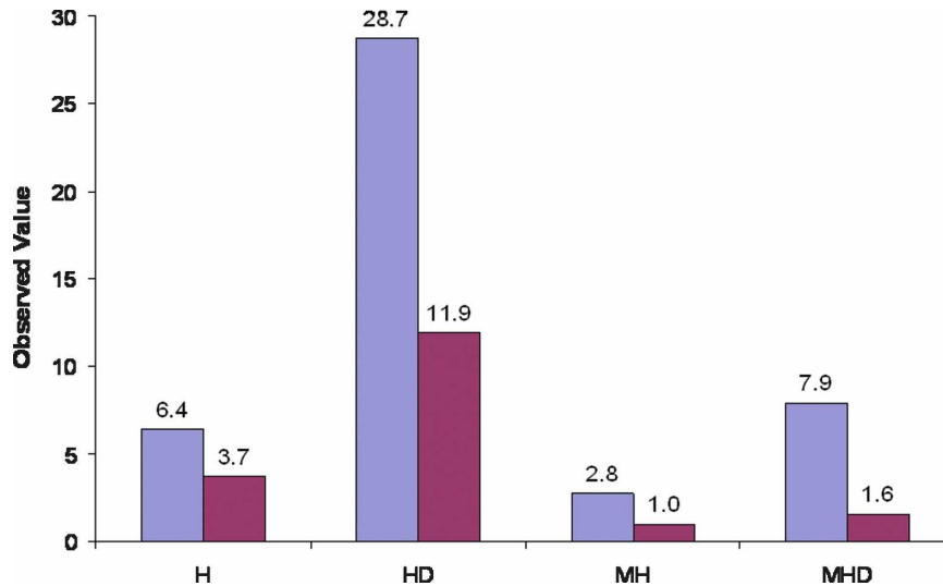
FIG. 2. Annually averaged Atlantic basin H, HD, MH, and MHD for the top 20 AMO years (blue bar) and the bottom 20 AMO years (red bar).
