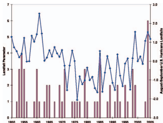
FIG. 6. The LP and Aug-Sep U.S. hurricane landfalls for 1950–2005 LP are the blue solid line, and Aug-Sep U.S. hurricane landfalls are the red columns. Note that, in general, more landfalls occur when LP values are above average.
