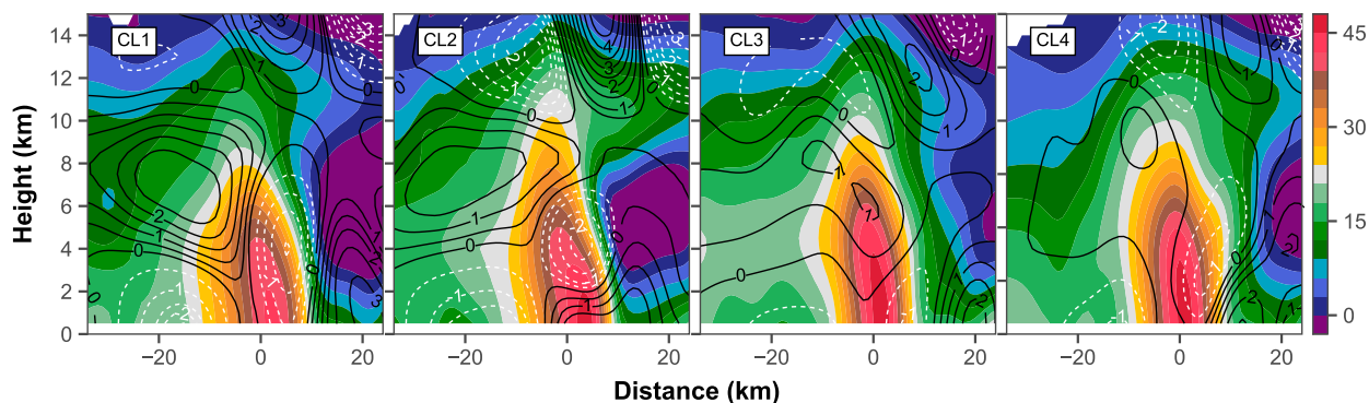
FIG. 15. Radial advection of AAM (contour) overlaid on the reflectivity (color) averaged along the subbands. The values are contoured every 0.5 \times 10^4 \text{ m}^2 \text{ s}^{-2} but labeled every 1 \times 10^4 \text{ m}^2 \text{ s}^{-2} for clarity.
