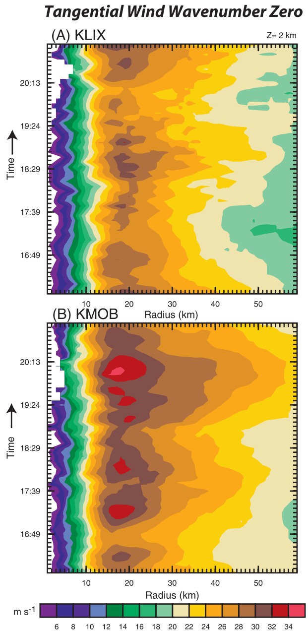
FIG. 10. Time–radius (Hovmöller) plot of GBVTD-derived mean tangential wind ( \text{m s}^{-1} ) wavenumber 0 for (a) KLIX and (b) KMOB.
