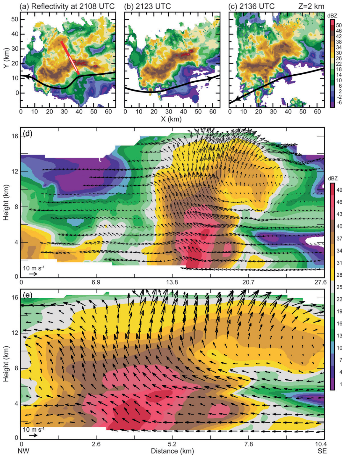
FIG. 8. (a)–(c) ELDORA radar reflectivity at the 2-km level for the three fly-bys of the intense convective cell. The times indicate the beginning of the 10–15-min passes by the convective feature. (d) Vertical cross section from northwest (NW) to southeast (SE) along the longer (red) line of (a). (e) Vertical cross section along the shorter (white) line of (a). Cartesian domains are relative to National Hurricane Center best-track position of Ophelia at 0000 UTC 7 Sep 2005.
