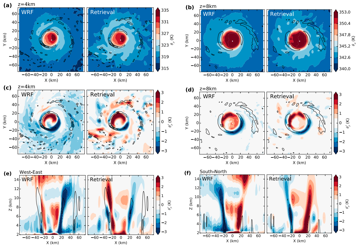
FIG. 5. Comparison of WRF output and temperature retrieval output for 1800 UTC 21 Sep 2005 as in Fig. 4.
