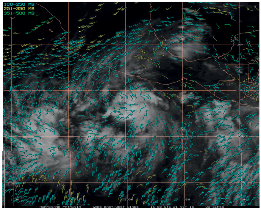
FIG. 6. Upper-level satellite-derived winds ( \text{m s}^{-1} ) on GOES IR imagery centered on Patricia at 1800 UTC 21 Oct 2015. Flag denotes wind speeds \sim 25 \text{ m s}^{-1} ; full barb denotes wind speeds \sim 5 \text{ m s}^{-1} ; half barb denotes wind speeds \sim 2.5 \text{ m s}^{-1} . Blue barbs denote winds in the 100–250-hPa layer; yellow barbs are the 251–350-hPa layer; green barbs are 351–500-hPa layer.
