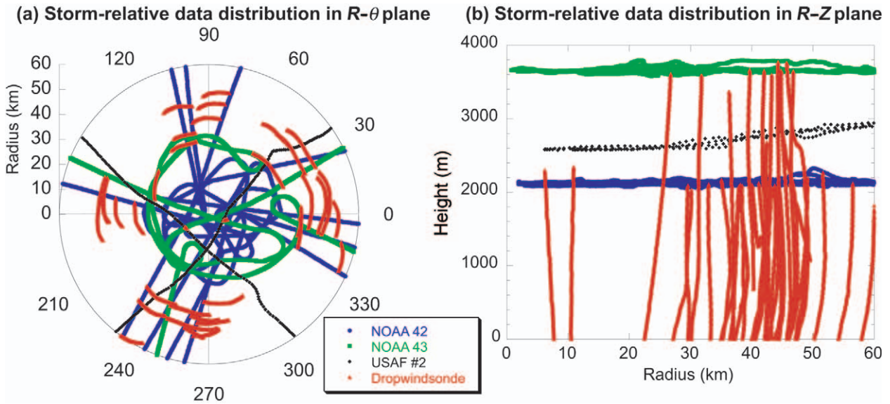
FIG. 2. Dropwindsonde locations and trajectories and aircraft flight tracks relative to storm center from 1600 to 2300 UTC 13 Sep. Storm-relative data distribution in the (a) radius–azimuthal ( R-\theta ) plane and (b) radius–height ( R-Z ) plane, showing the NOAA P-3 (42 in blue, 43 in green) and USAF C-130 (in black) flight tracks, and dropwindsonde trajectories (in red). The dropwindsondes in (a) move cyclonically (counterclockwise).
