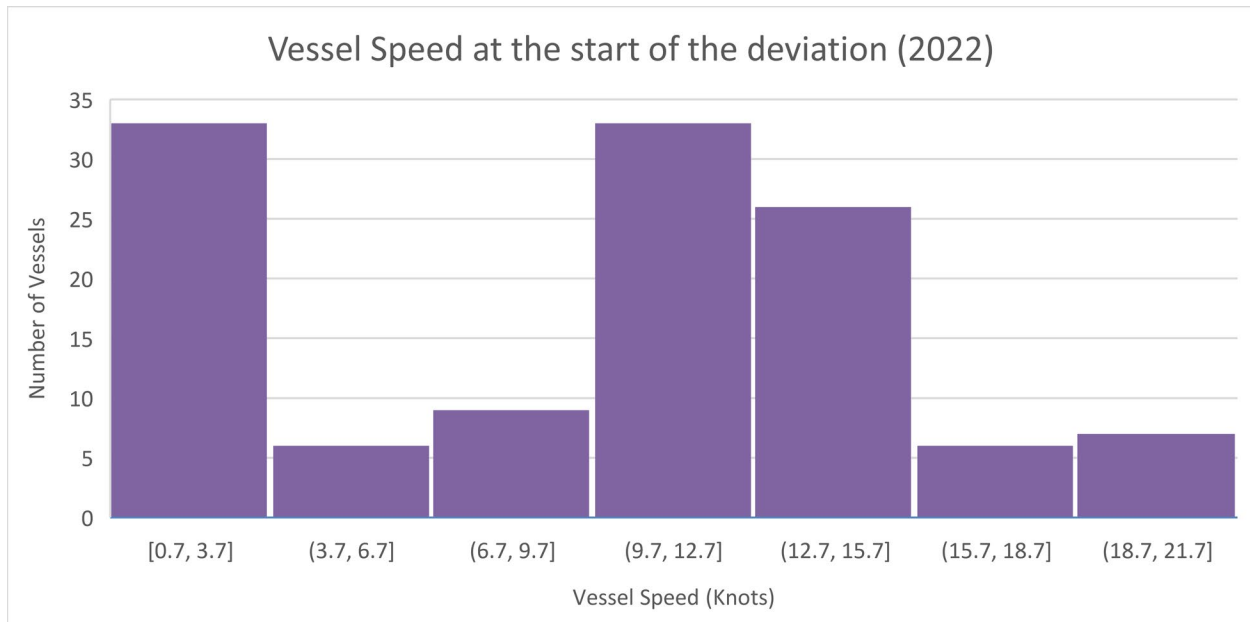
Figure 18. Histogram of vessel speed while first deviating according to 2022 AIS data provided by Marine Traffic (binned in 3 knots but dependent on lowest speed at the start of deviation per year).
