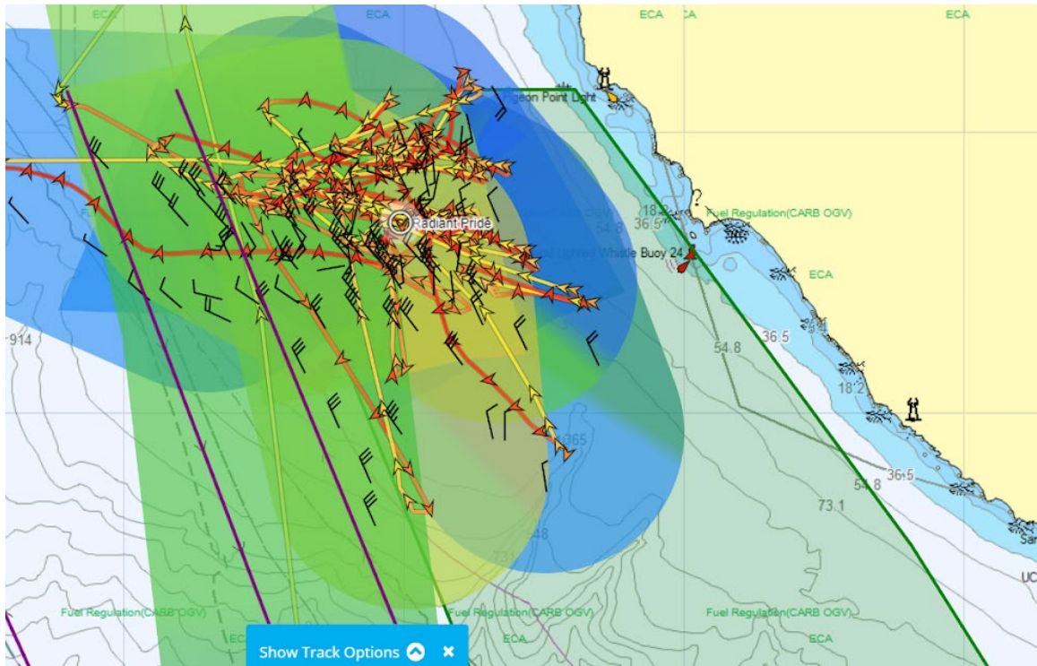
Figure 8. Vessel tracking back and forth over the northern area of the IMO recommended tracks (purple lines) and within the customized alert zone (green box) in April 2022. Wind bars are also shown.
