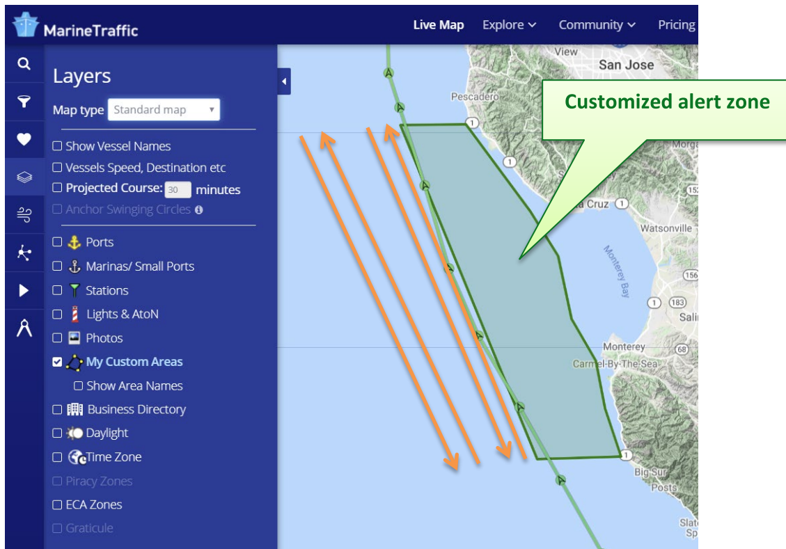
Figure 7. A vessel track of a deviating vessel. The vessel's track is represented by the light green line and black arrows within green circles, which indicate when AIS data were received by AIS ground stations. The orange lines represent the IMO recommended tracks. This track shows the vessel entered the customized alert zone, (i.e. the deviation area represented by the light green area with dark green outline) twice, clipping area corners at both Point Sur and Pigeon Point. This event would prompt Marine Traffic to send two (2) email notifications, but only the first email notification details would be entered into the spreadsheet because the same vessel conducted both deviations. However, both notifications would be copied and pasted into each Google Doc linked to the spreadsheet for the deviation record.
