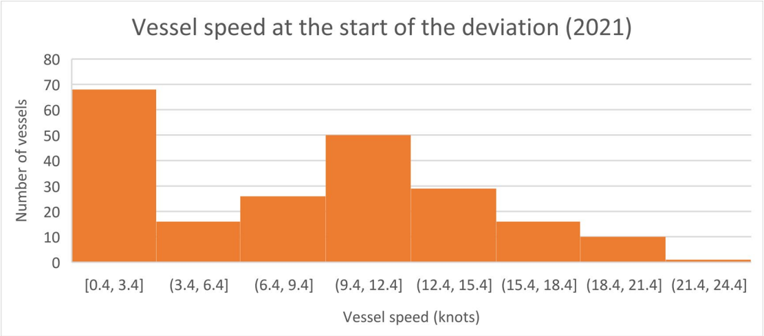
Figure 17. Histogram of vessel speed while first deviating according to 2021 AIS data provided by Marine Traffic (binned in 3 knots but dependent on lowest speed at the start of deviation per year).
