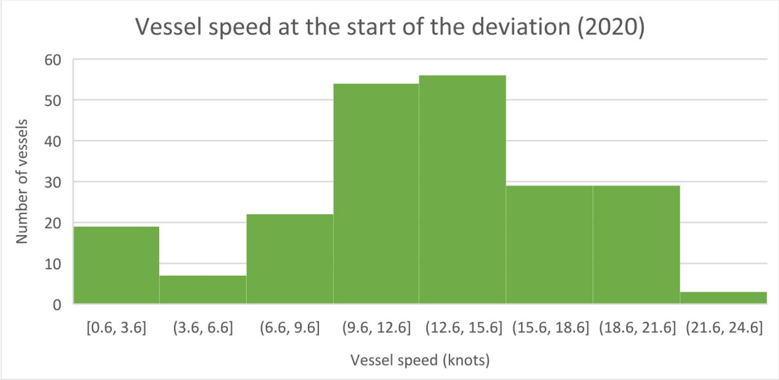
Figure 16. Histogram of vessel speed while first deviating according to 2020 AIS data provided by Marine Traffic (binned in 3 knots but dependent on lowest speed at the start of deviation per year).
