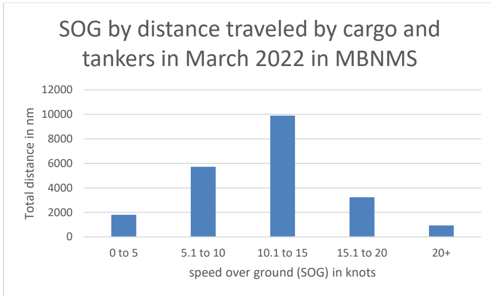
Figure 20. Speed over ground (SOG) by distance in March 2022 in MBNMS
