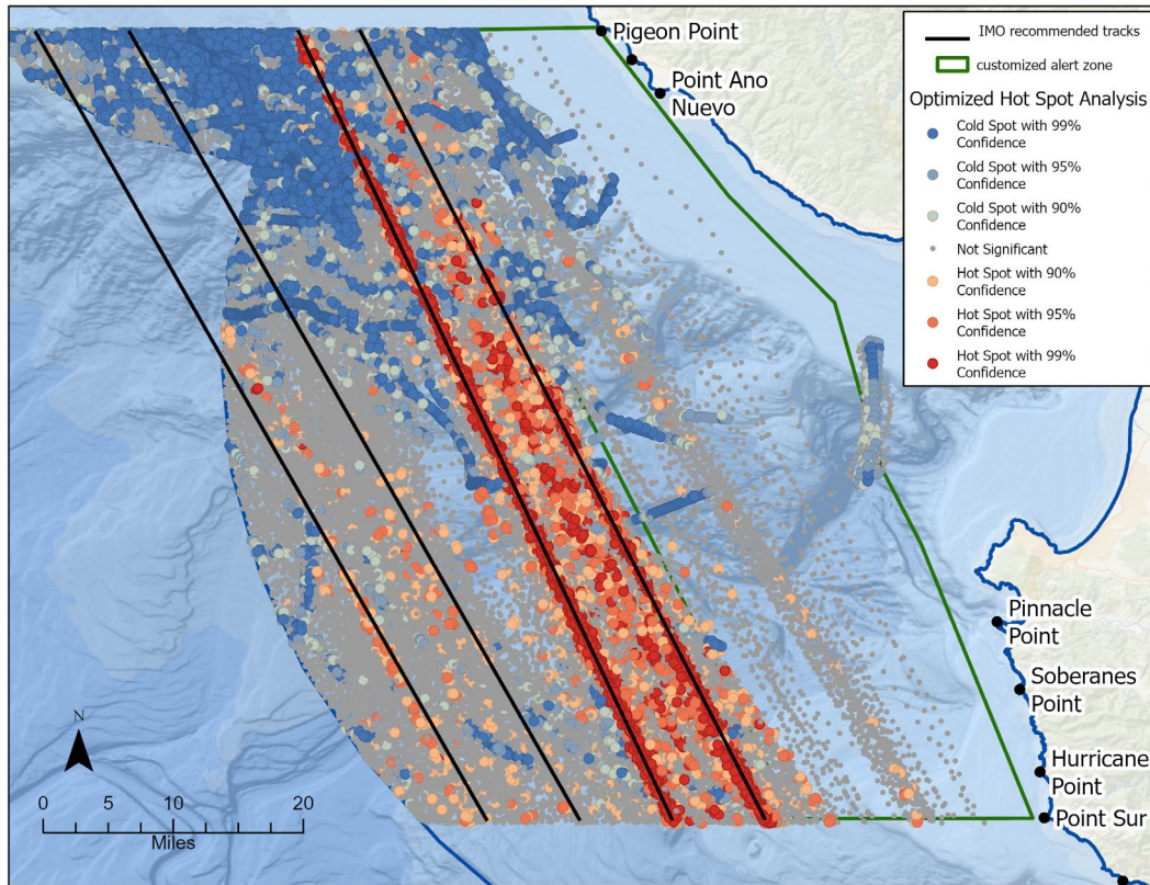
Figure 19. Optimized Hot Spot Analysis to show hot spots where high vessel speeds (red features) of tankers and cargo vessels are clustered and where low vessel speeds (blue features) are clustered while transiting through MBNMS in 2020.
