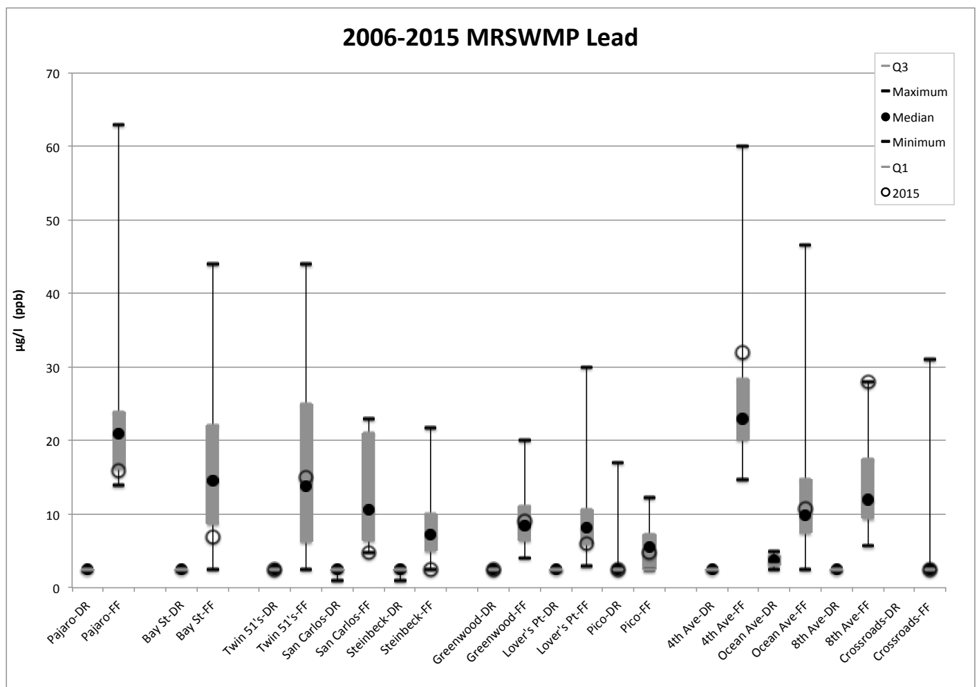
Figure 11. 2006-2015 MRSWMP lead results. Non-detects were given the value of half the Minimum Detection Limit (MDL) but their true value lies between the zero and the MDL. Sites are listed north to south.
