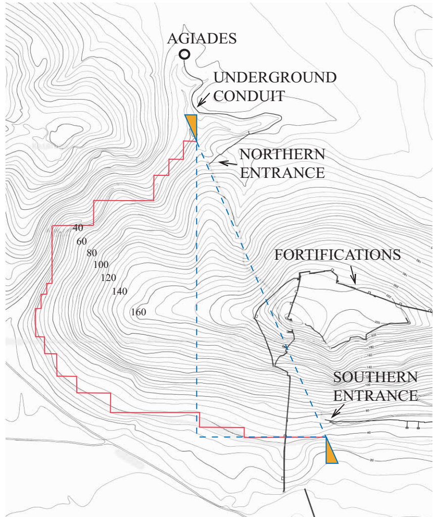
This schematic diagram shows how Hero's method can be applied to the terrain on Samos. The hypotenuse of the large right triangle is the line of the proposed tunnel. Markers can be put along the hypotenuses of the small right triangles at each entrance to help the tunnelers dig in the right direction.
